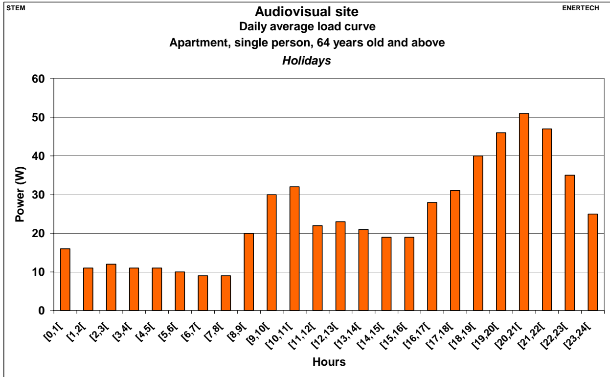
Figure 2.397: Audiovisual site – Daily average load curve – Apartment, single person, 64 years old and above – Holidays
