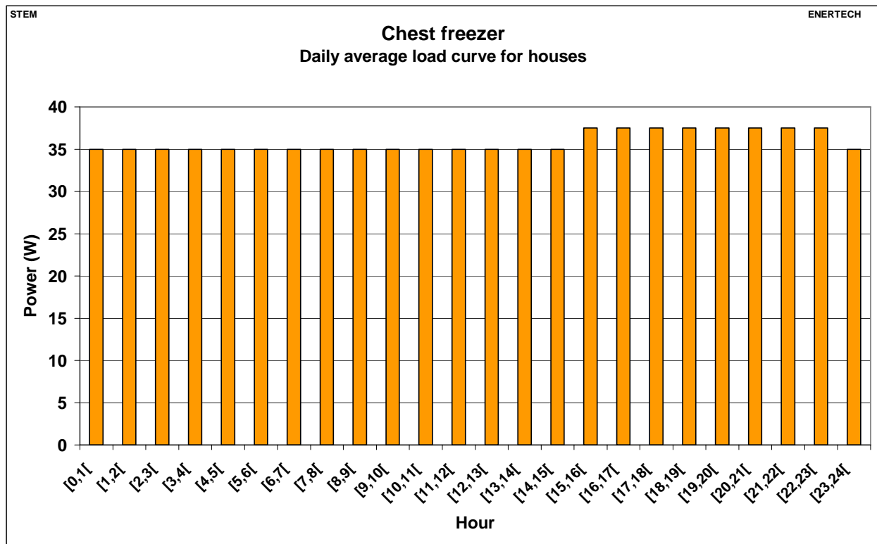
Figure 2.206: Chest freezer: daily average load curves – all households
