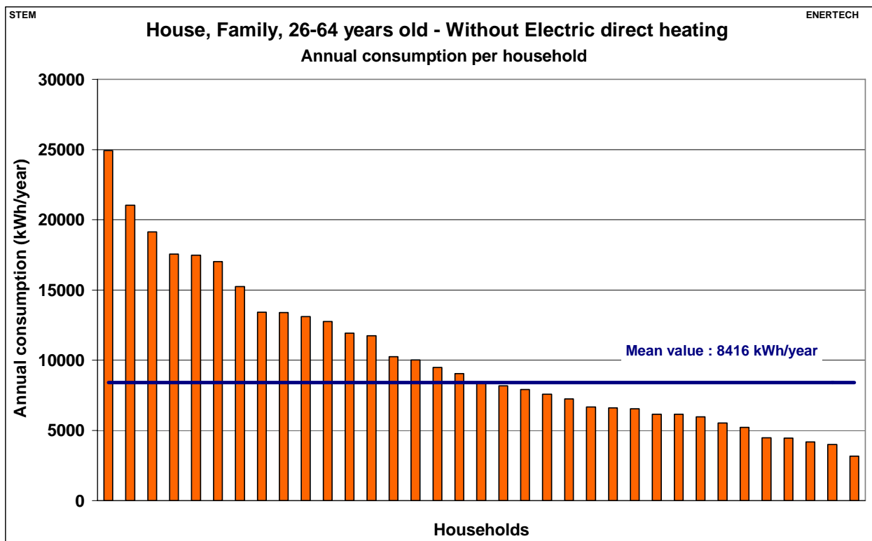
Figures 2.4: Total annualized electricity consumption – Houses without electric heating
