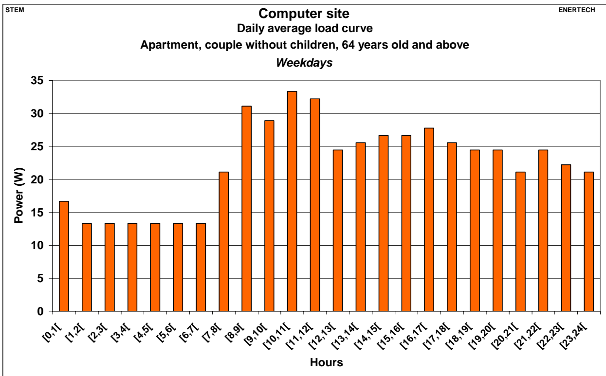
Figure 2.431: Computer site – Daily average load curve – Apartment, couples without children, 64 years old and above – Weekdays
