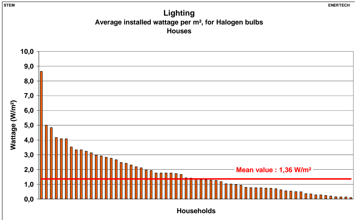
Figure 2.332: Lighting – Average installed wattage per m 2 for halogen bulbs – Houses
