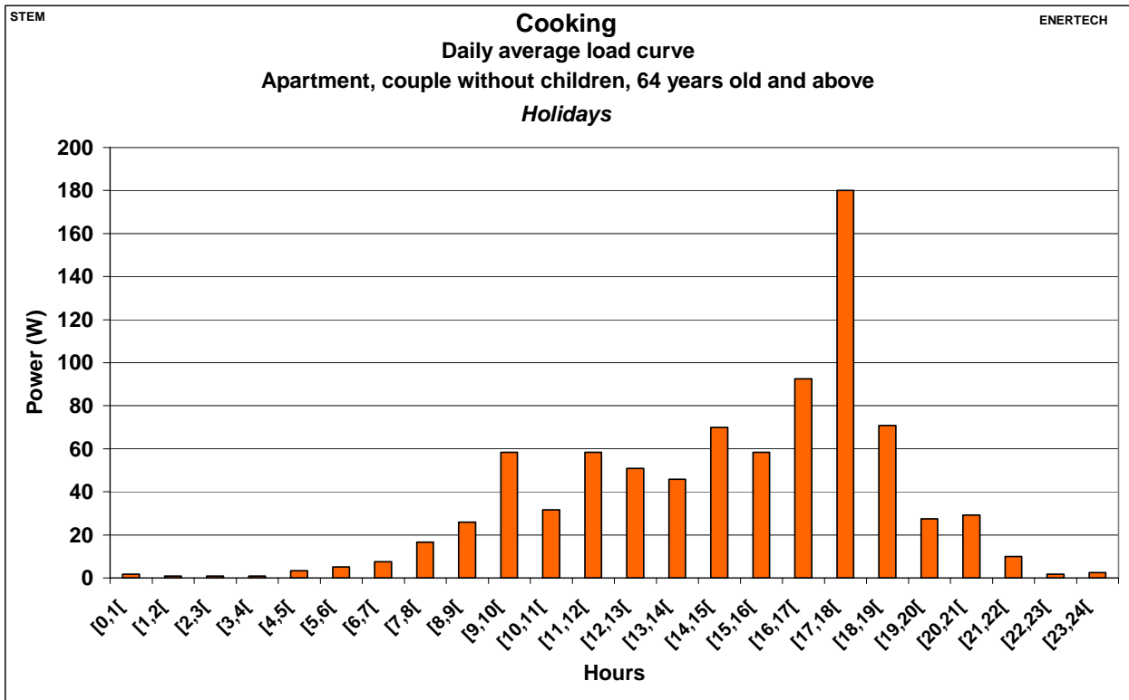
Figure 2.276: Cooking – Daily average load curve – Apartment, couples without children, 64 years old and above – Holidays
