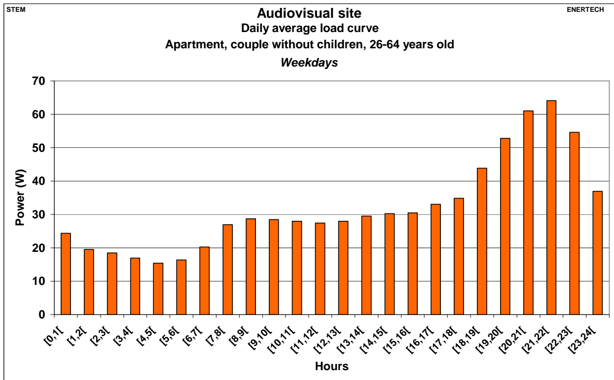
Figure 2.390: Audiovisual site – Daily average load curve – Apartment, couples without children, 26-64 years old – Weekdays
