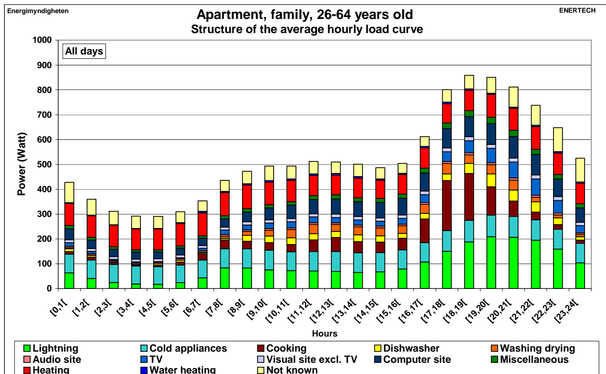
Figure 2.68: Structure of the average hourly load curve – Apartments - All days
