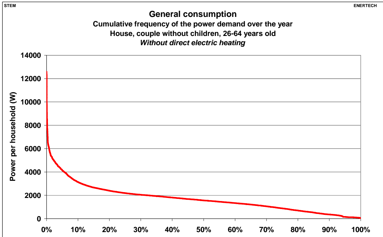
Figure 2.48: General consumption – Cumulative frequency of the power demand over the year, from the grid point of view – House, couples without children, 26-64 years old – Without direct electric heating
