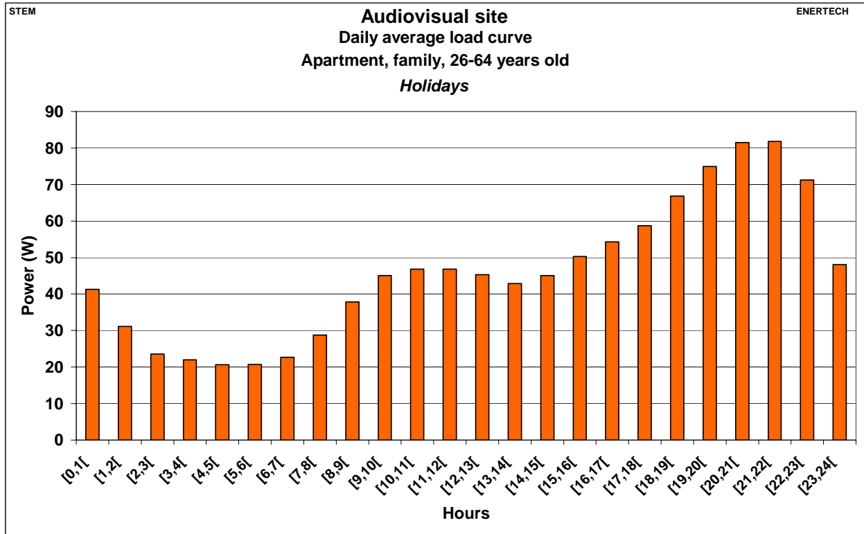
Figure 2.393: Audiovisual site – Daily average load curve – Apartment, family, 26-64 years old – Holidays
