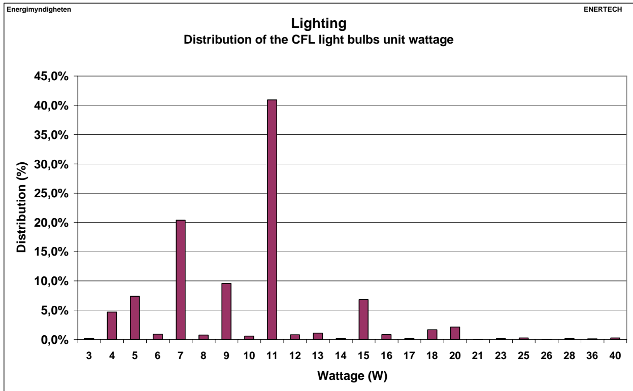
Figure 2.341: Lighting – Distribution of the CFL light bulbs unit wattage
