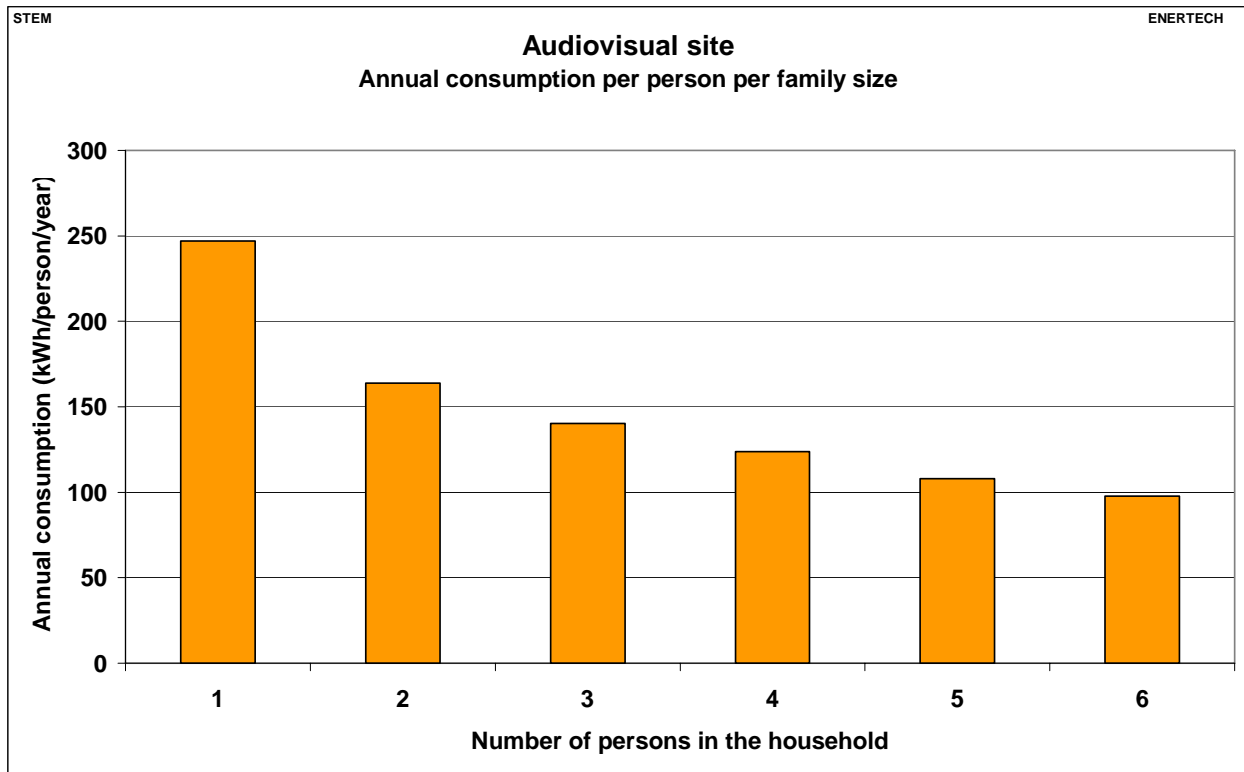
Figure 2.388: Audiovisual site – Annual consumption per person per family size
