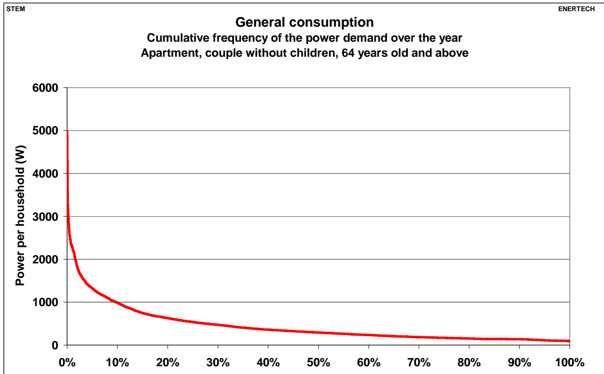
Figure 2.52: General consumption – Cumulative frequency of the power demand over the year, from the grid point of view – Apartment, couples without children, 64 years old and above
