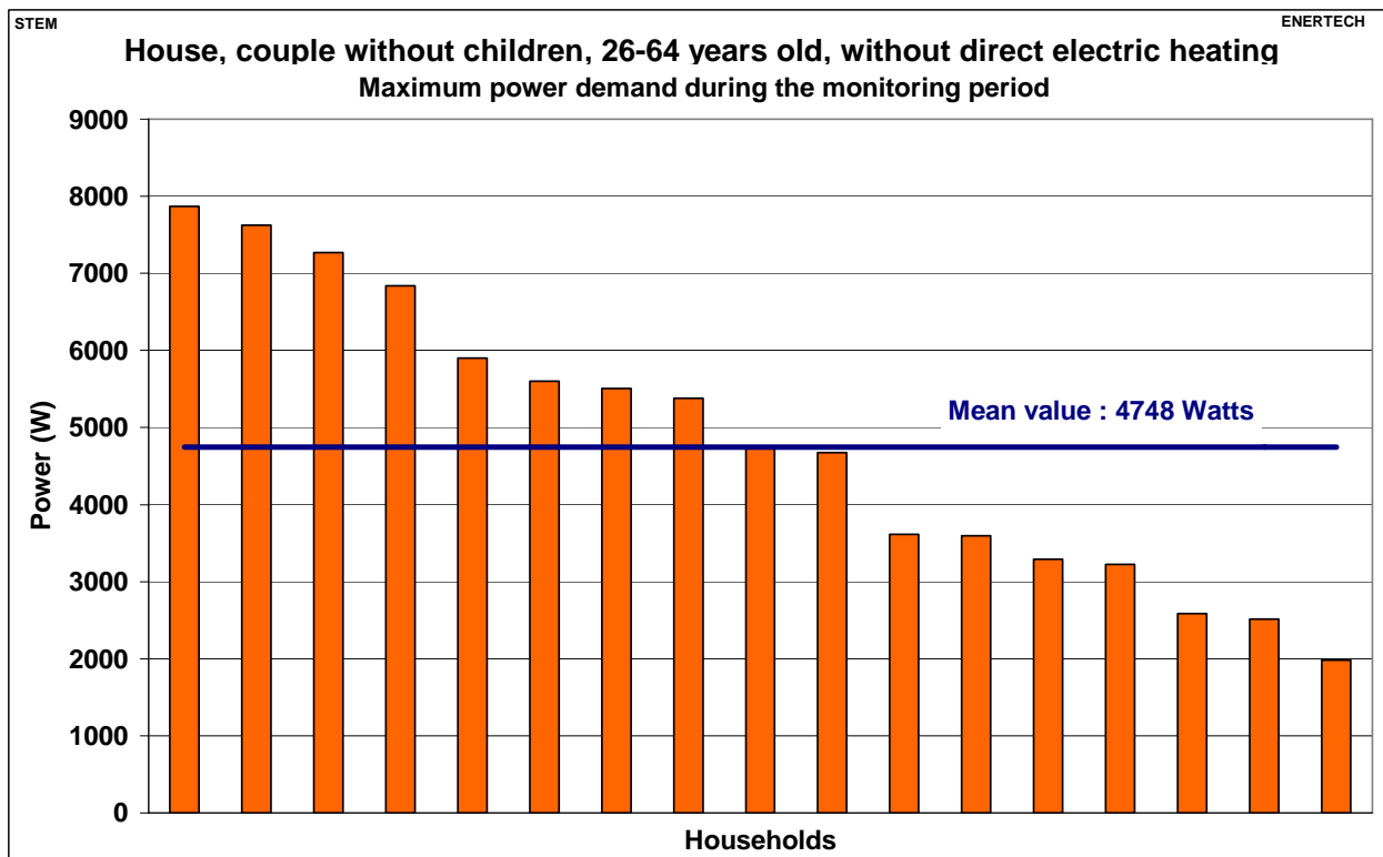
Figure 2.37: Maximum power demand – Houses without direct electric heating
