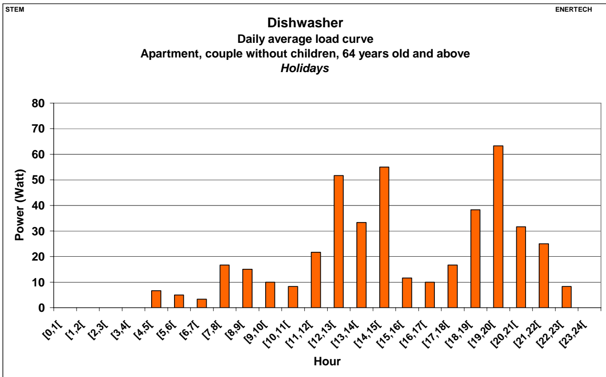
Figure 2.251: Dishwasher – Daily average load curve – Apartment, couples without children, 64 years old and above– Holidays
