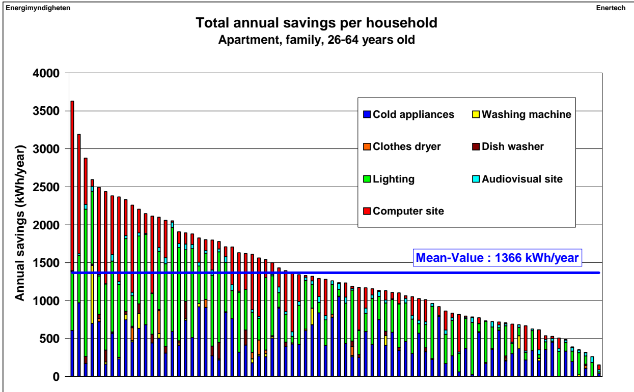
Figure 3.18: Total annual savings per household – Apartment, family, 26-64 years old
