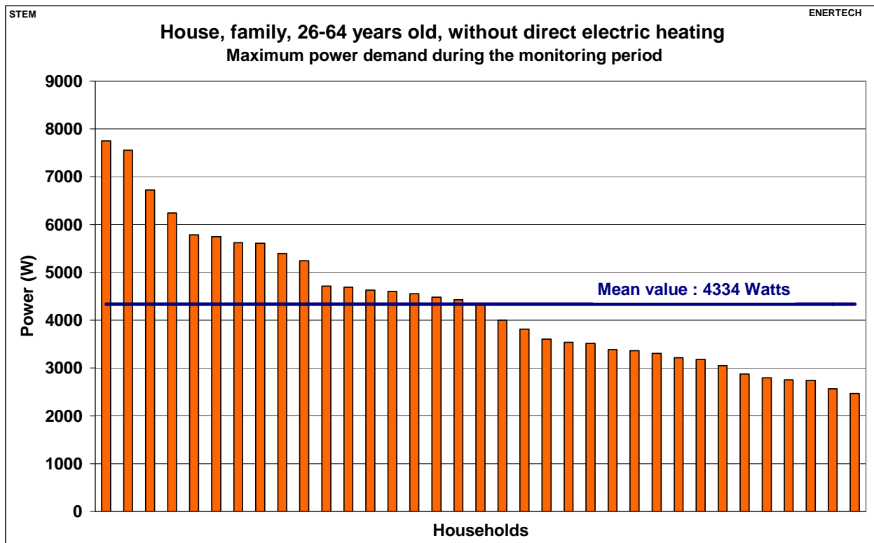
Figure 2.34: Maximum power demand – Houses without direct electric heating
