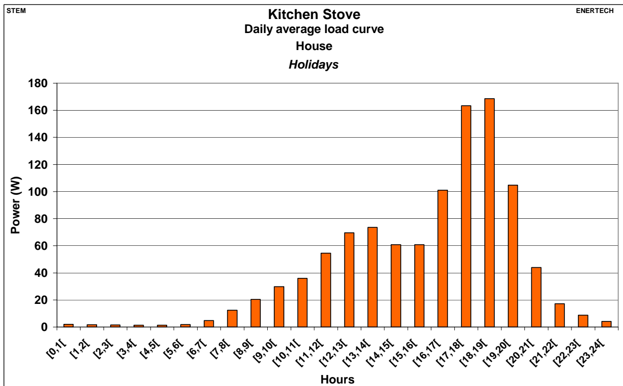
Figure 2.302: Kitchen Stove – Daily average load curve – Houses – Holidays
