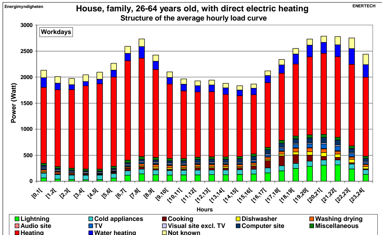
Figure 2.58: Structure of the average hourly load curve – Houses with direct electric heating – Workdays
