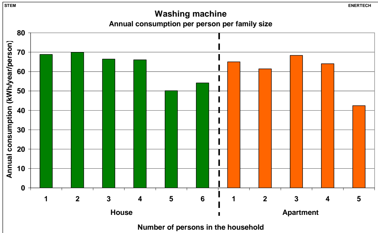
Figure 2.213: Washing machine: annual consumption per person per household size
