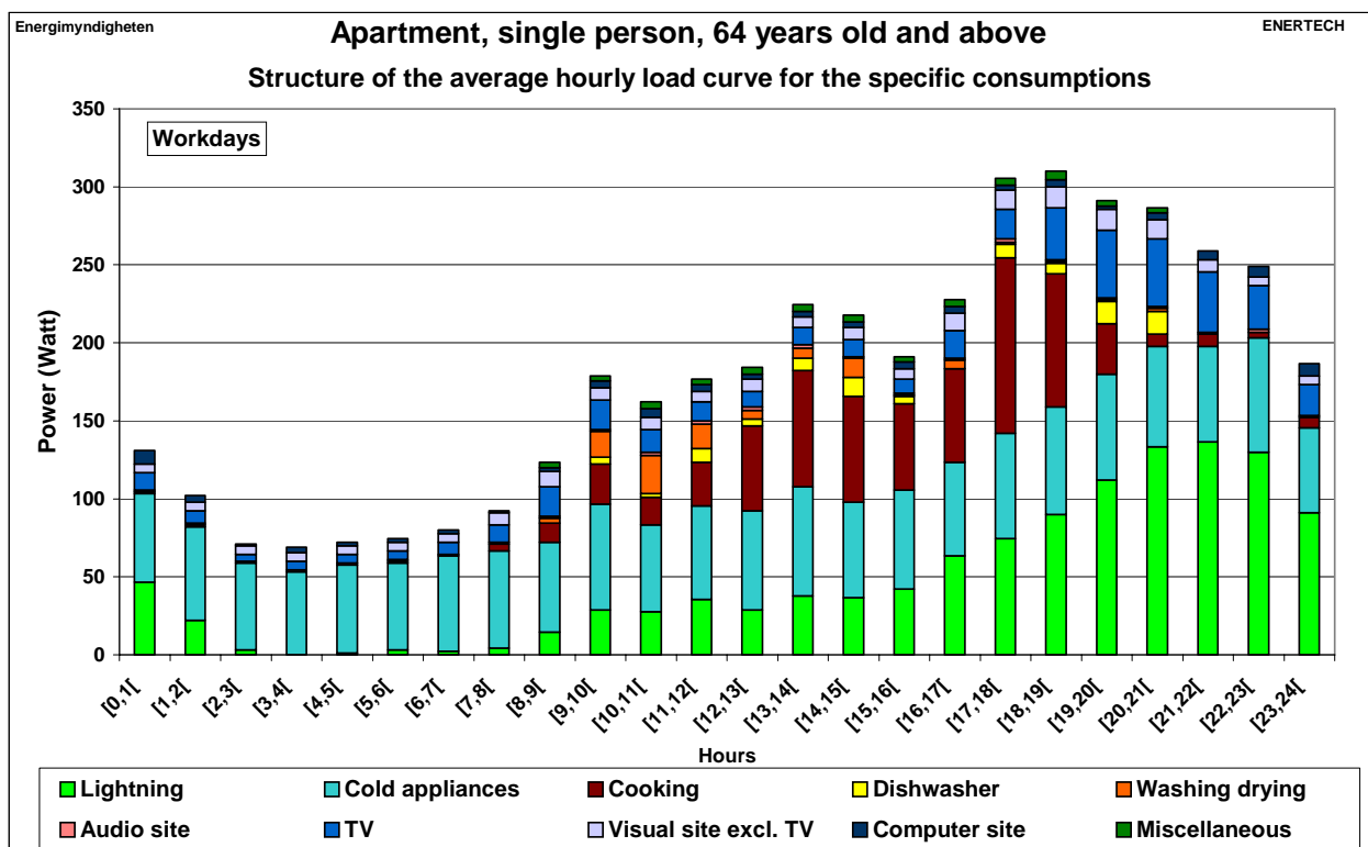
Figure 2.121: Structure of the average hourly load curve for the specific consumption– Apartments – Workdays
