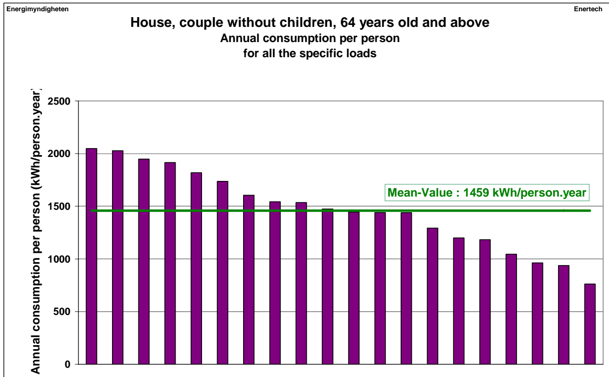
Figures 2.24-D: Total annualized electricity consumption per person – Specific consumption only - Houses
