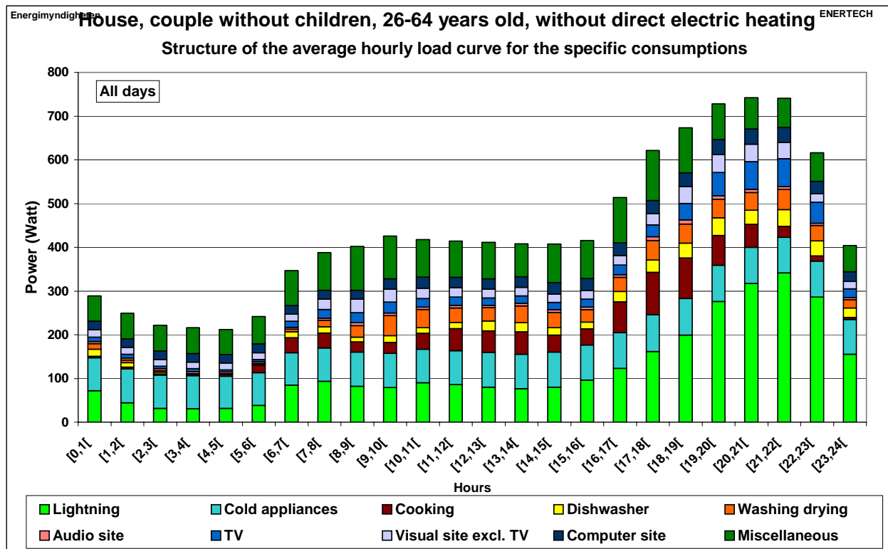
Figure 2.83: Structure of the average hourly load curve for the specific consumption– Houses without direct electric heating – All days
