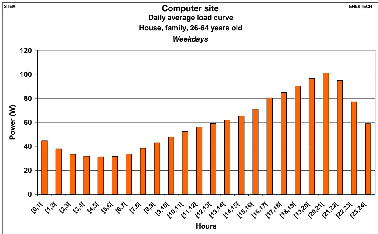
Figure 2.443: Computer site – Daily average load curve – House, family, 26-64 years old – Weekdays
