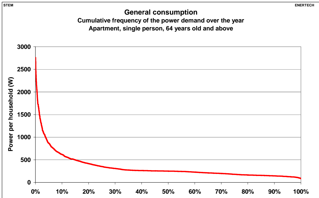
Figure 2.54: General consumption – Cumulative frequency of the power demand over the year, from the grid point of view – Apartment, single person, 64 years old and above
