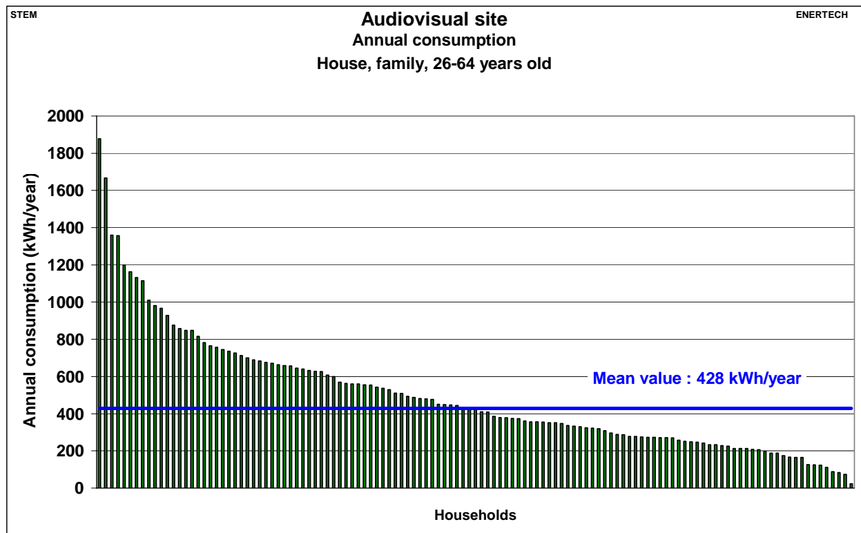
Figure 2.381: Audiovisual site – Annual consumption – House, family, 26-64 years old
