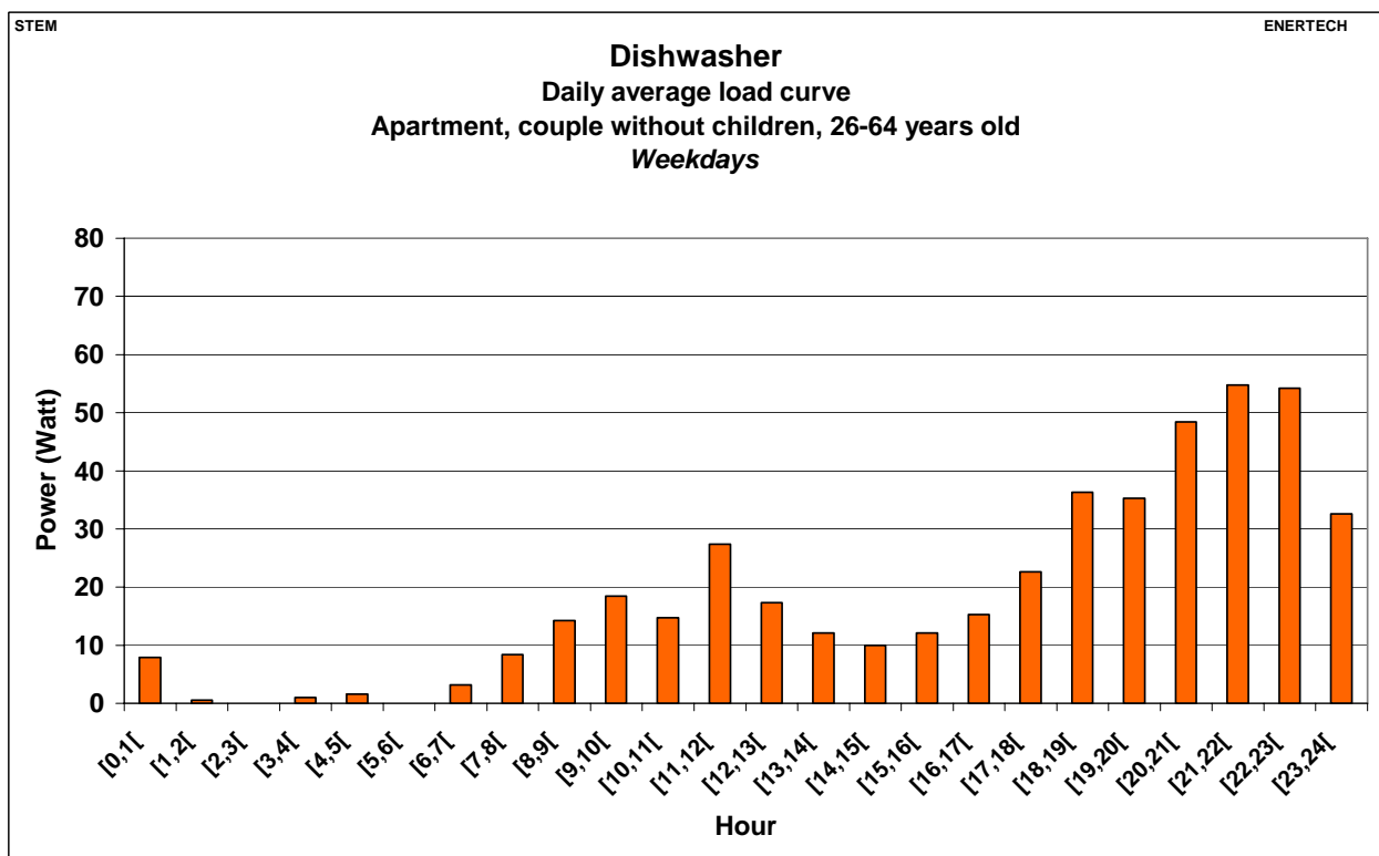
Figure 2.250: Dishwasher – Daily average load curve – Apartment, couples without children, 26-64 years old – Weekdays
