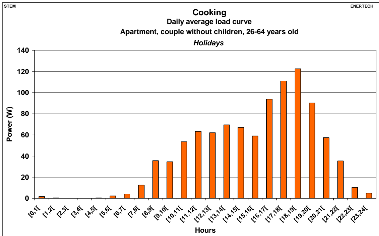
Figure 2.274: Cooking – Daily average load curve – Apartment, couples without children, 26-64 years old – Holidays
