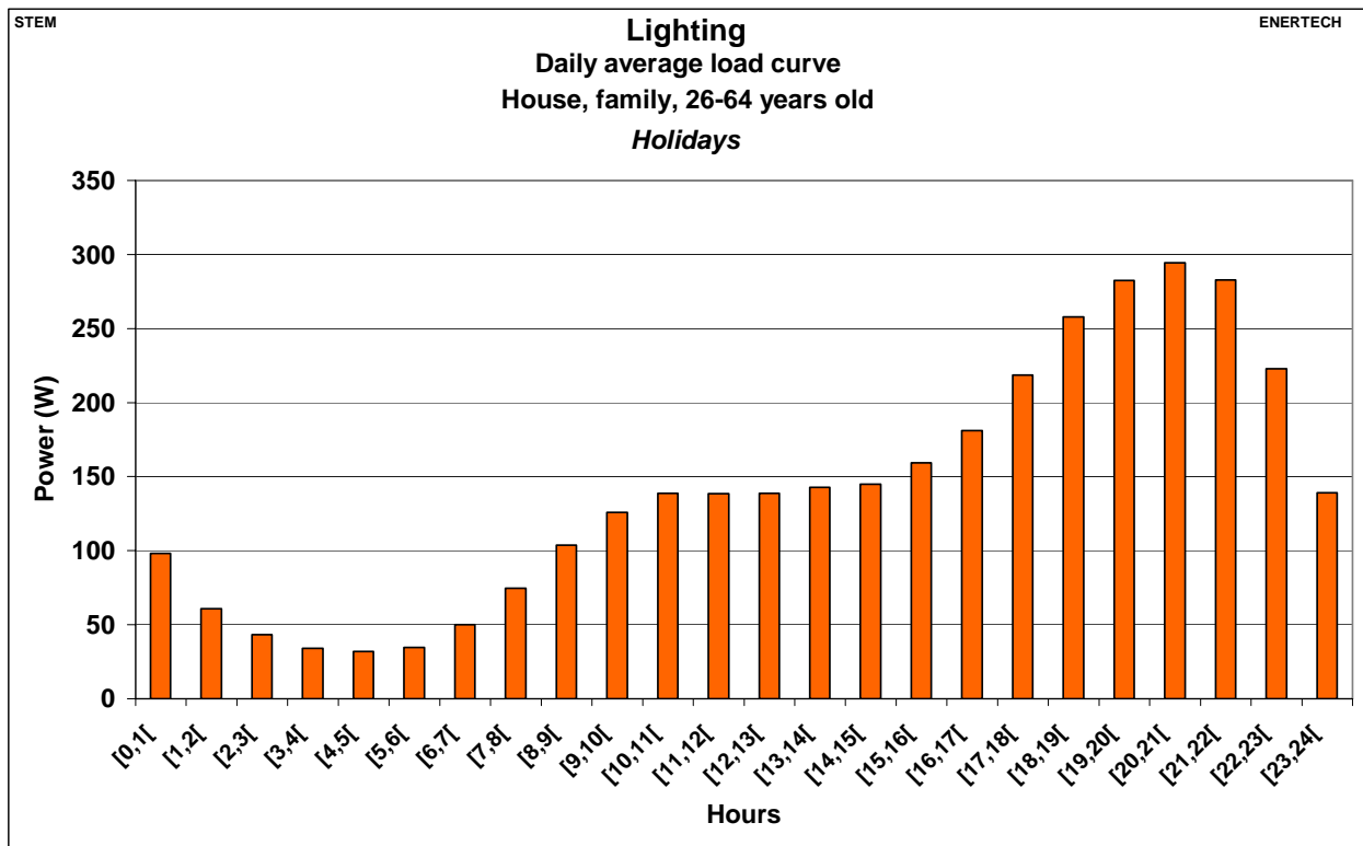
Figure 2.375: Lighting – Daily average load curve – House, family, 26-64 years old – Holidays
