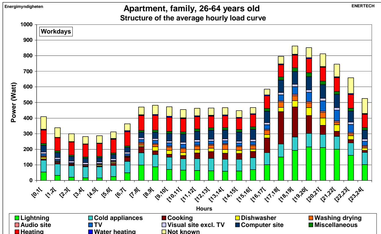
Figure 2.70: Structure of the average hourly load curve – Apartments - Workdays
