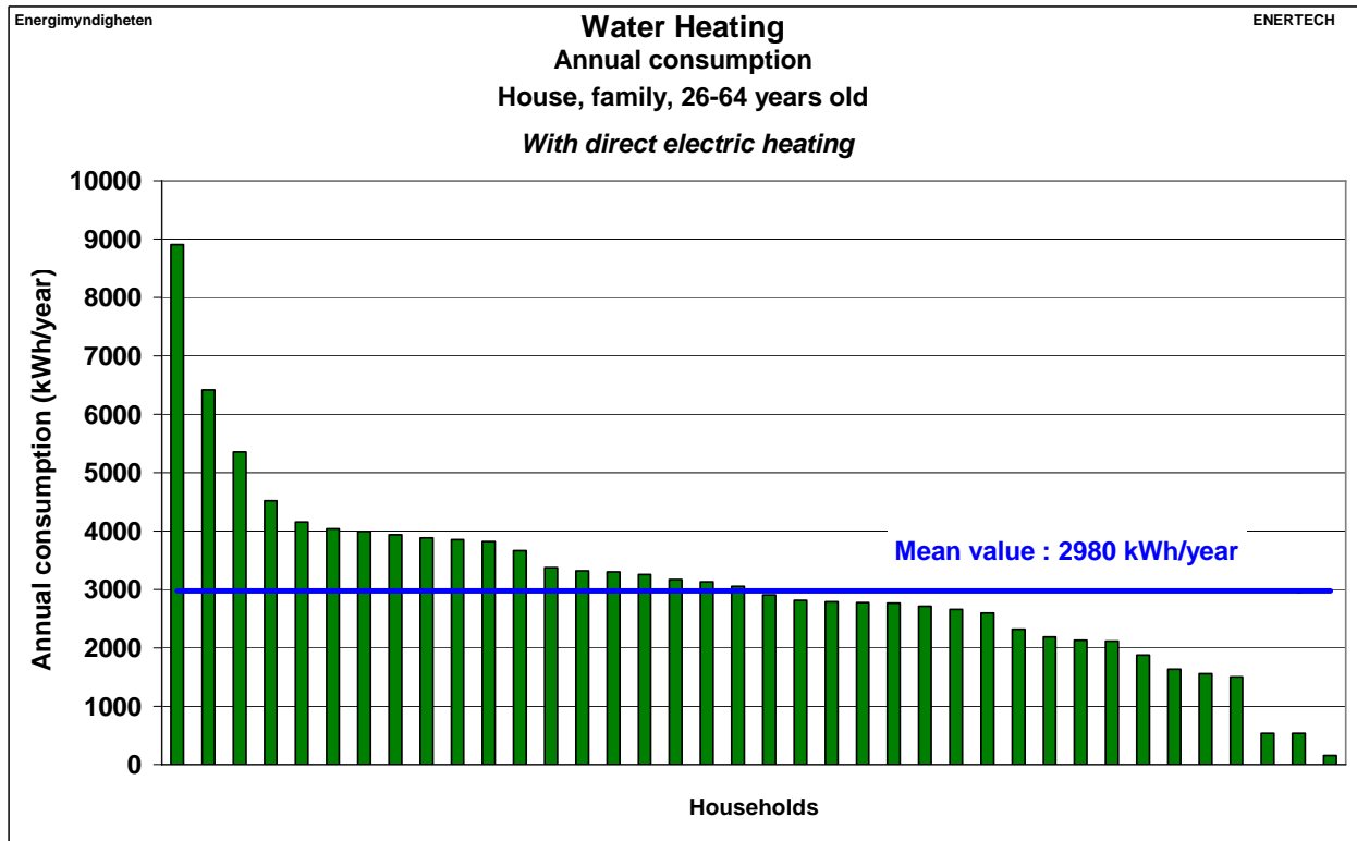
Figure 2.455: Water heating – Annual consumption – House, family, 26-64 years old –Direct electric heating
