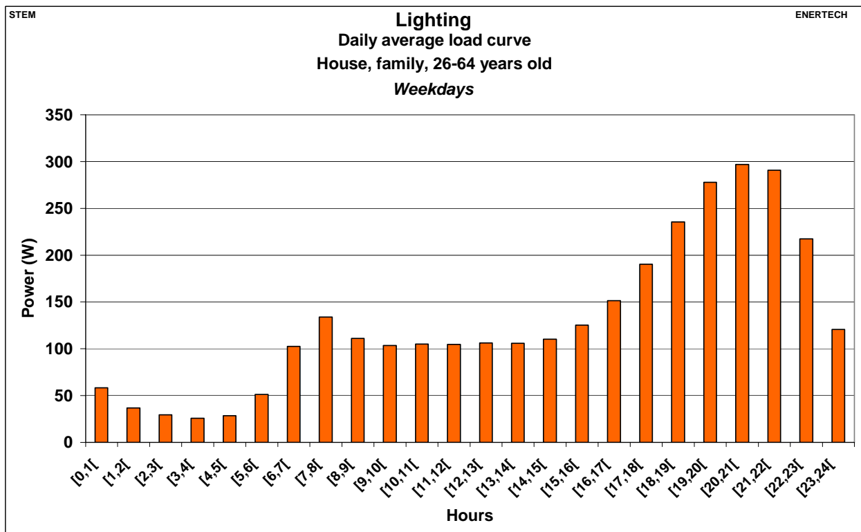
Figure 2.376: Lighting – Daily average load curve – House, family, 26-64 years old – Weekdays
