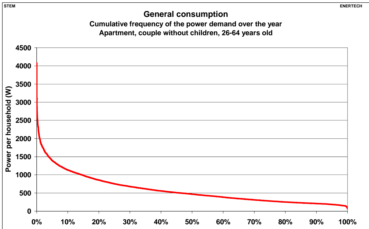
Figure 2.49: General consumption – Cumulative frequency of the power demand over the year, from the grid point of view – Apartment, couples without children, 26-64 years old
