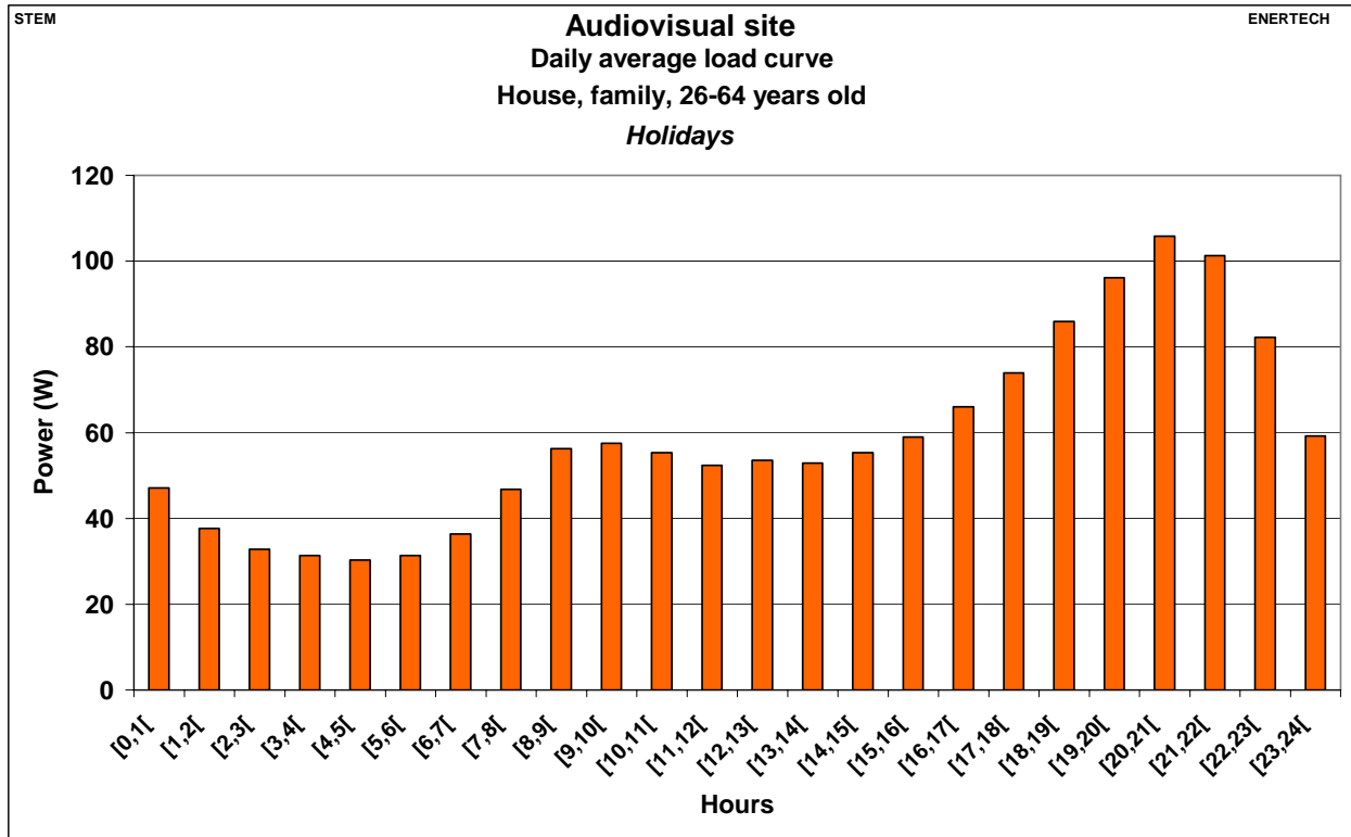
Figure 2.403: Audiovisual site – Daily average load curve – House, family, 26-64 years old – Holidays
