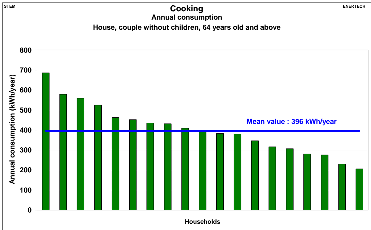
Figure 2.266: Cooking – Annual consumption – House, couples without children, 64 years old and above
