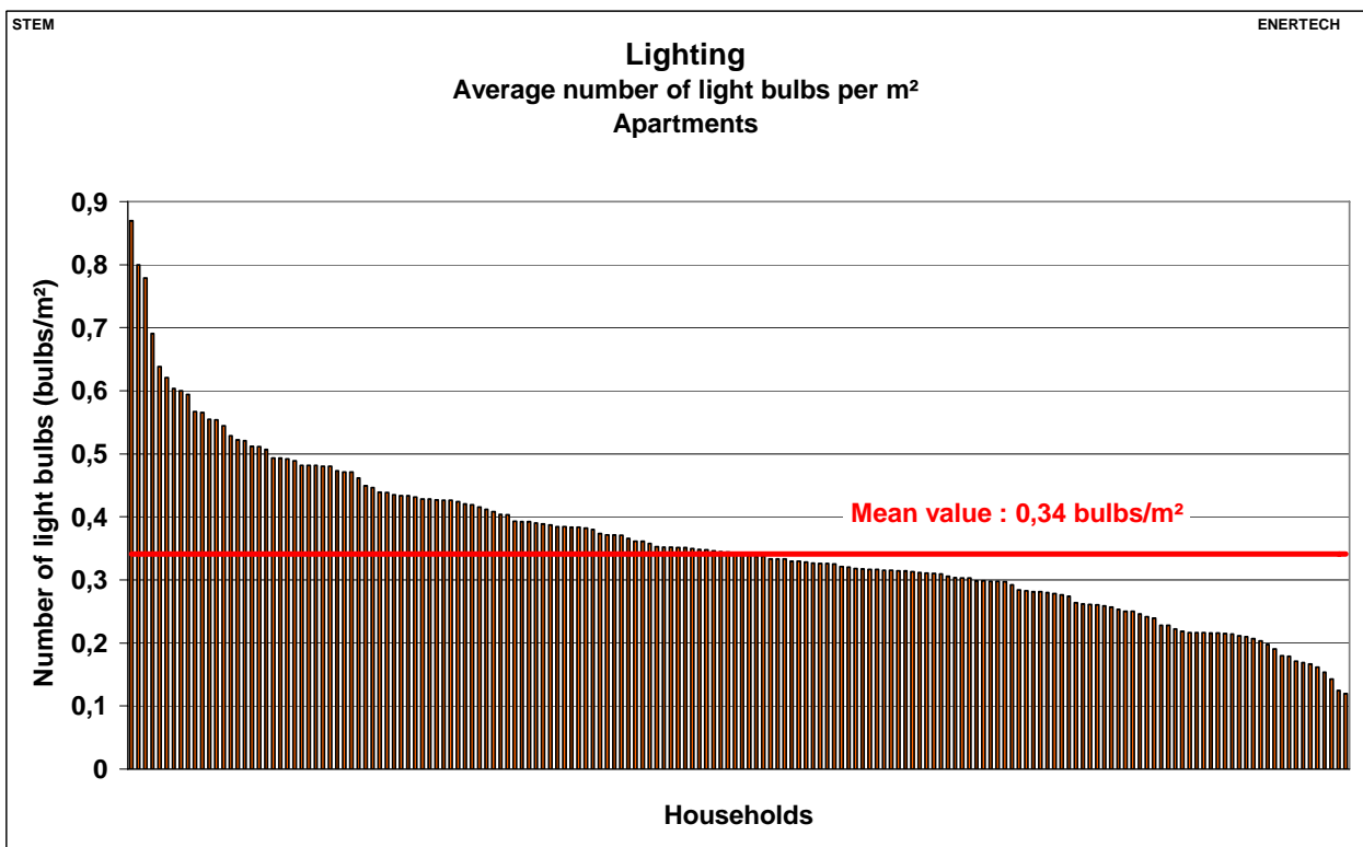
Figure 2.320: Lighting – Number of light bulbs per m 2 - Apartments
