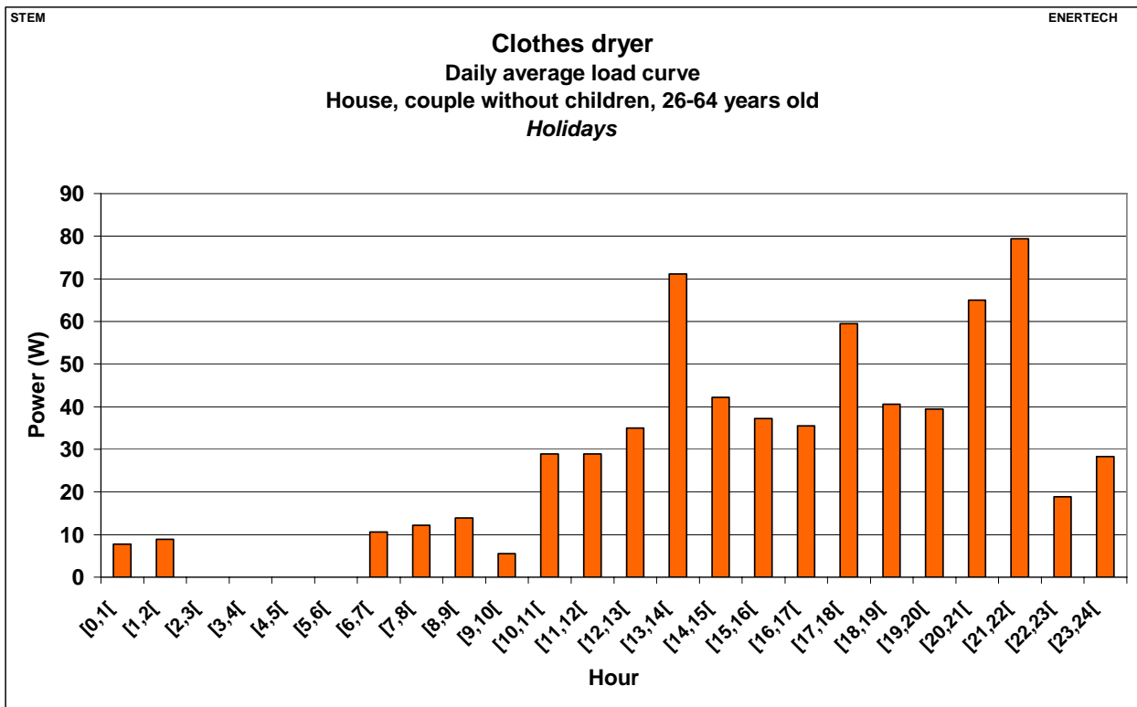
Figure 2.234: Clothes dryer – Daily average load curve – House, couples without children, 26-64 years old – Holidays
