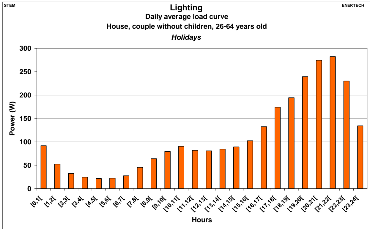
Figure 2.371: Lighting – Daily average load curve – House, couples without children, 26-64 years old – Holidays
