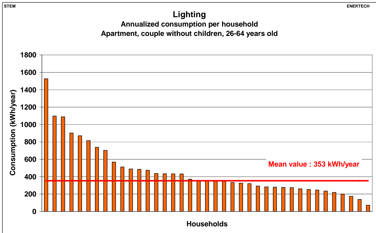
Figure 2.349: Lighting – Annualized consumption – Apartment, couples without children, 26-64 years old
