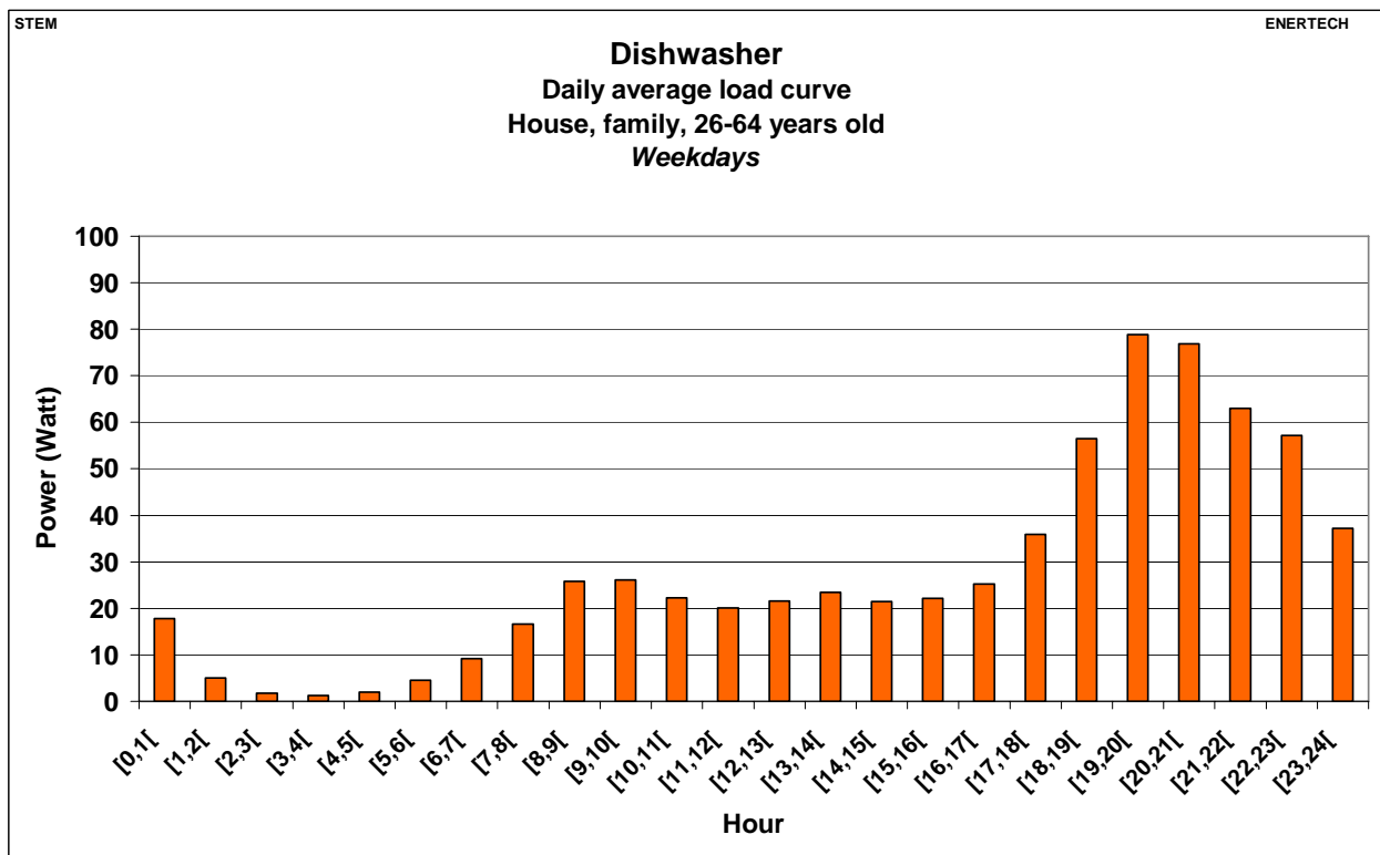
Figure 2.262: Dishwasher – Daily average load curve – House, family, 26-64 years old – Weekdays
