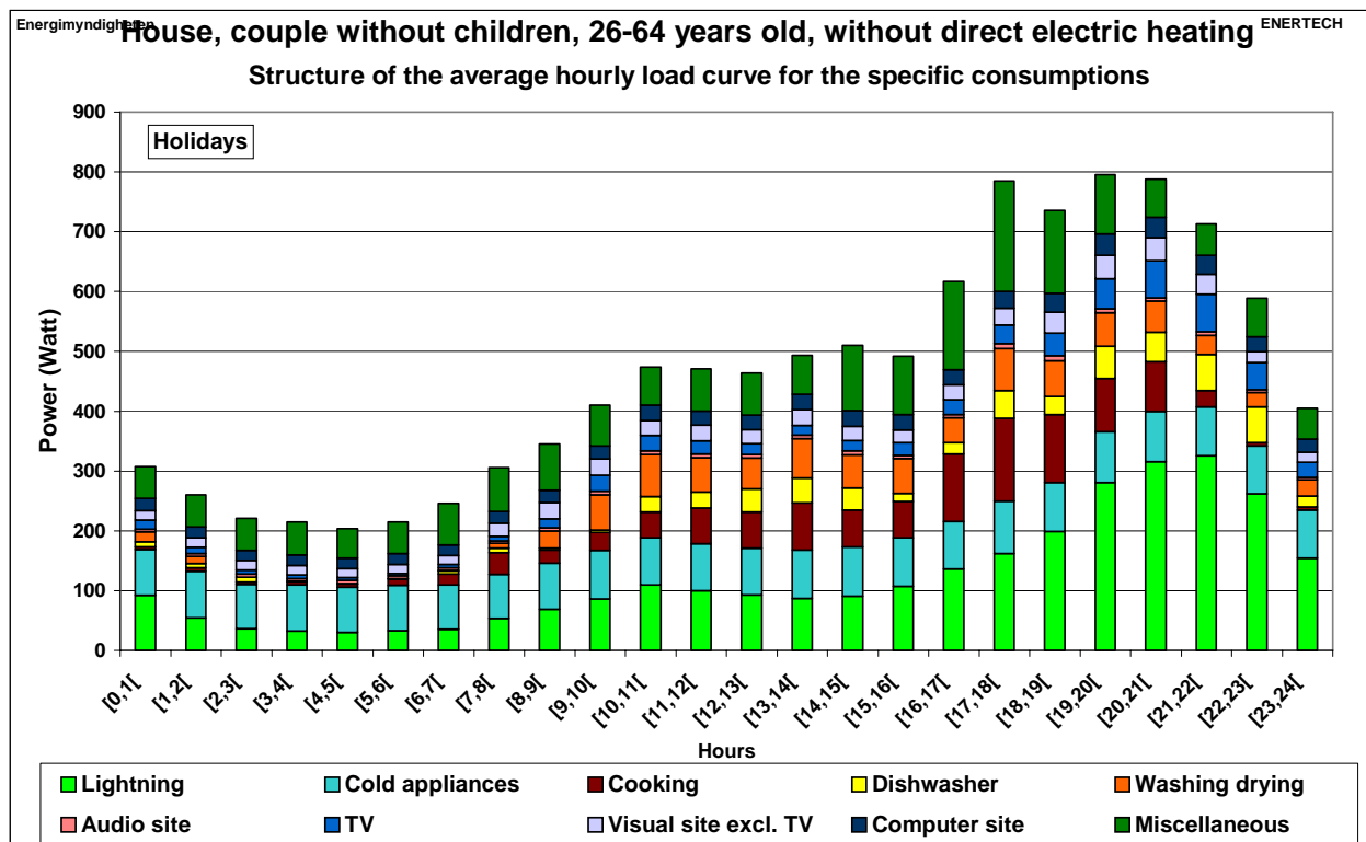
Figure 2.84: Structure of the average hourly load curve for the specific consumption– Houses without direct electric heating – Holidays
