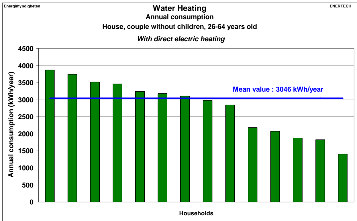
Figure 2.456: Water heating – Annual consumption – House, couples without children, 26-64 years old – Direct electric heating
