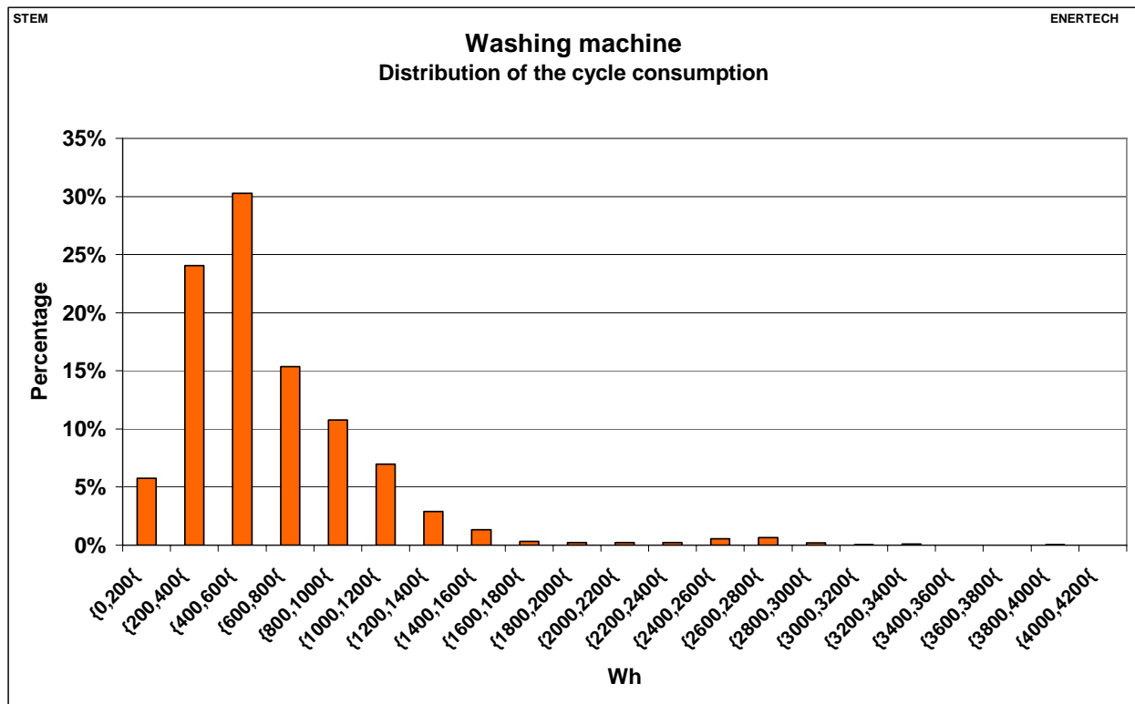
Figure 2.227: Washing machine – Distribution of the washing cycle consumption
