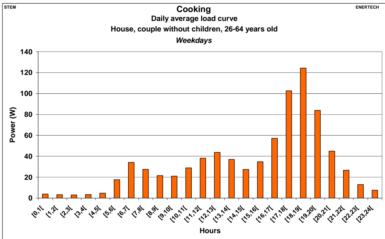
Figure 2.285: Cooking – Daily average load curve – House, couples without children, 26-64 years old – Weekdays
