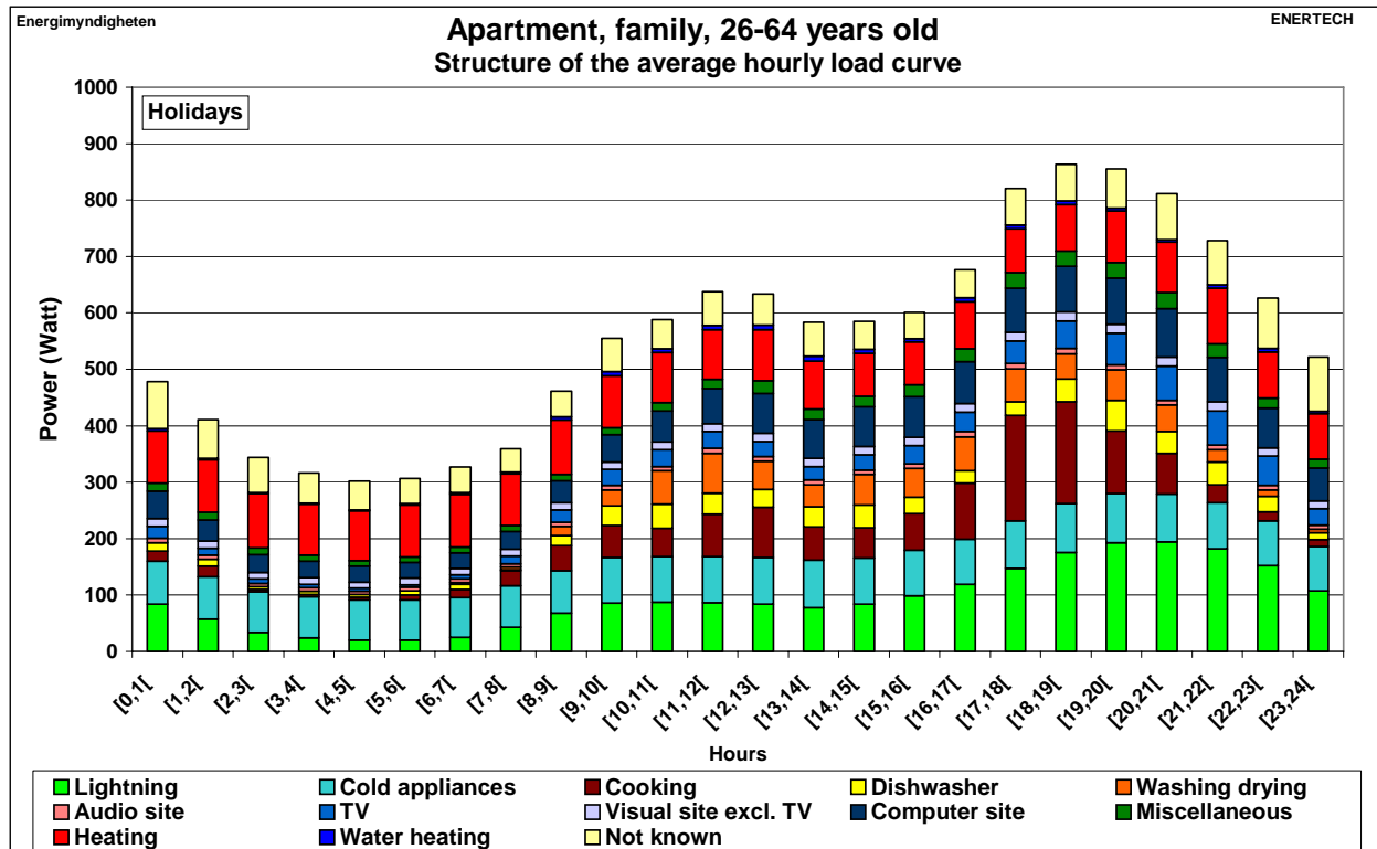
Figure 2.69: Structure of the average hourly load curve – Apartments - Holidays
