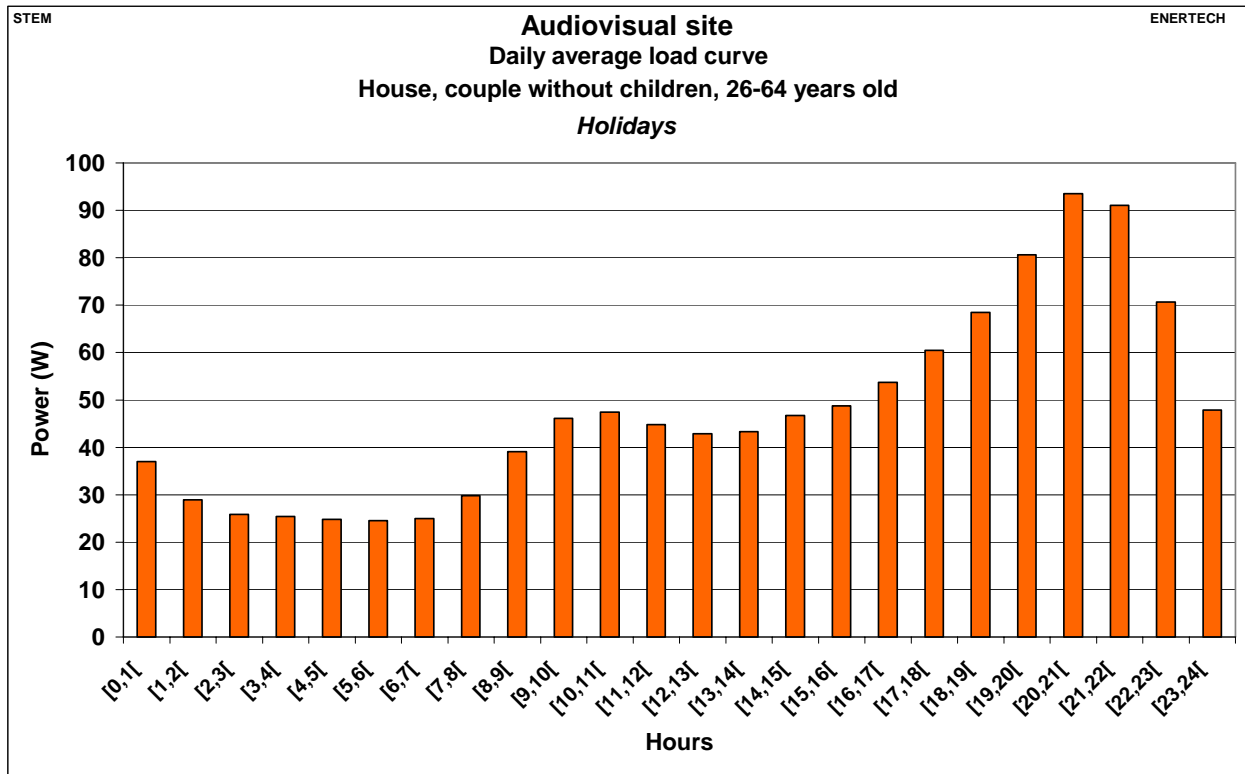
Figure 2.399: Audiovisual site – Daily average load curve – House, couples without children, 26-64 years old – Holidays
