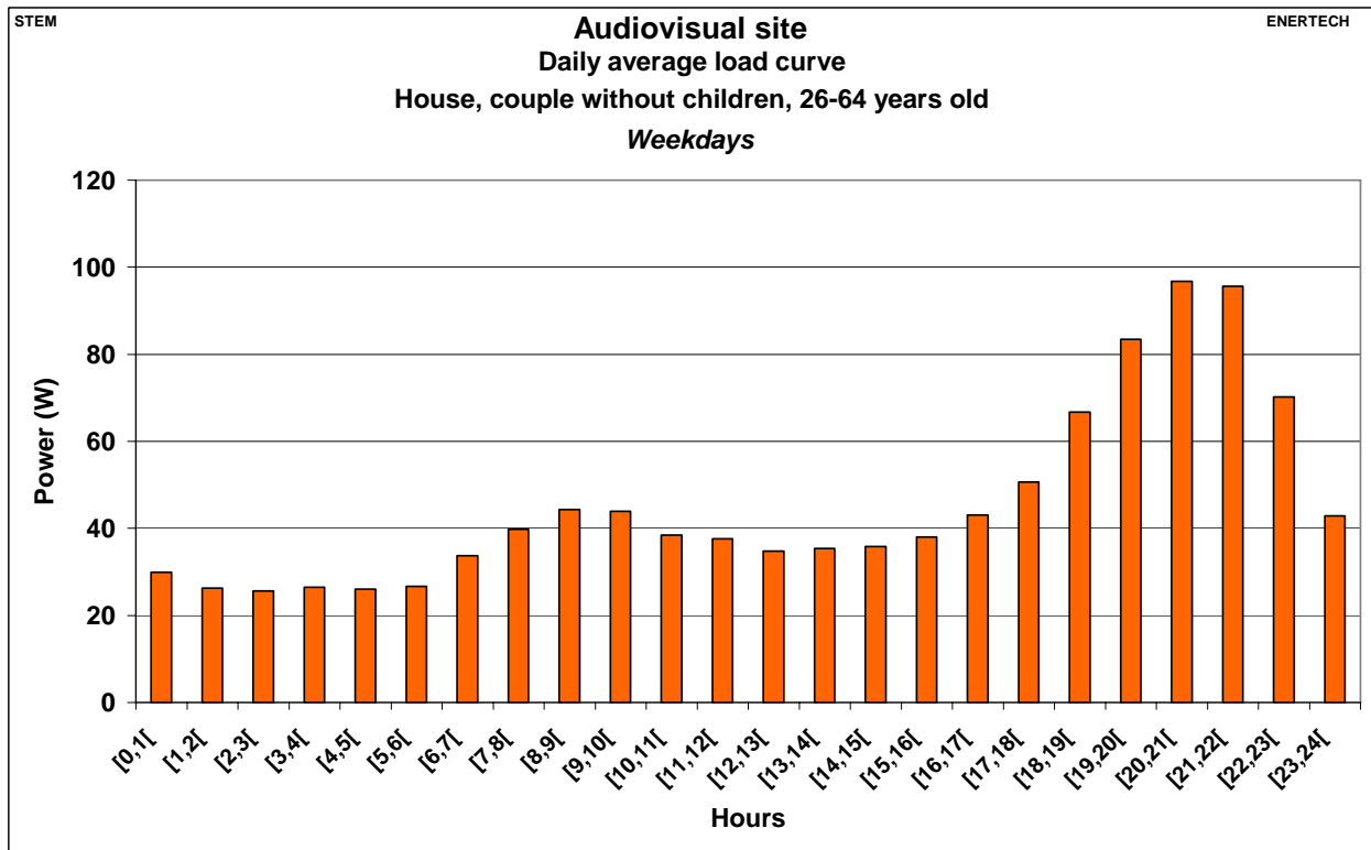
Figure 2.400: Audiovisual site – Daily average load curve – House, couples without children, 26-64 years old – Weekdays
