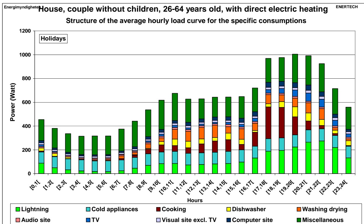
Figure 2.78: Structure of the average hourly load curve for the specific consumption– Houses with direct electric heating – Holidays
