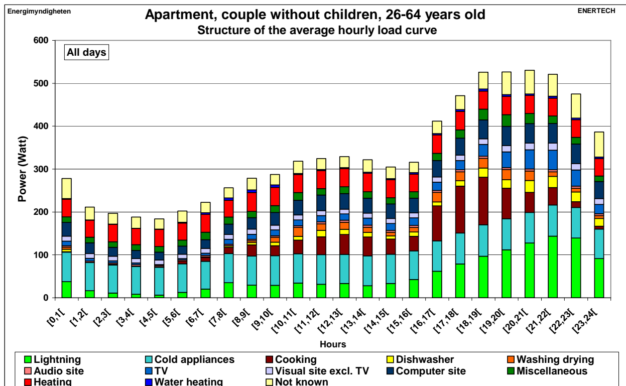
Figure 2.86: Structure of the average hourly load curve – Apartments – All days
