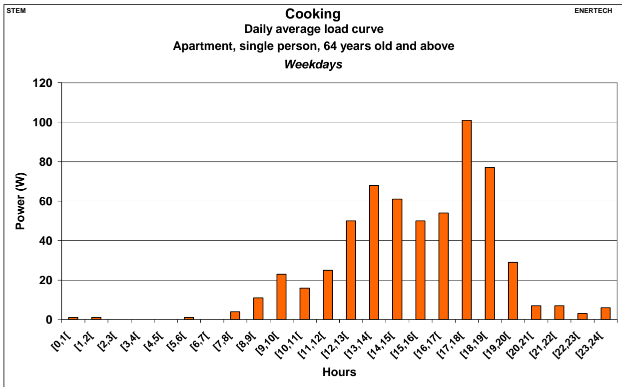
Figure 2.283: Cooking – Daily average load curve – Apartment, single person, 64 years old and above – Weekdays
