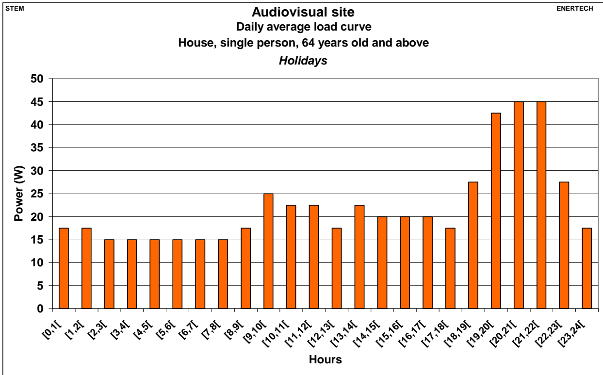
Figure 2.405: Audiovisual site – Daily average load curve – House, single person, 64 years old and above – Holidays
