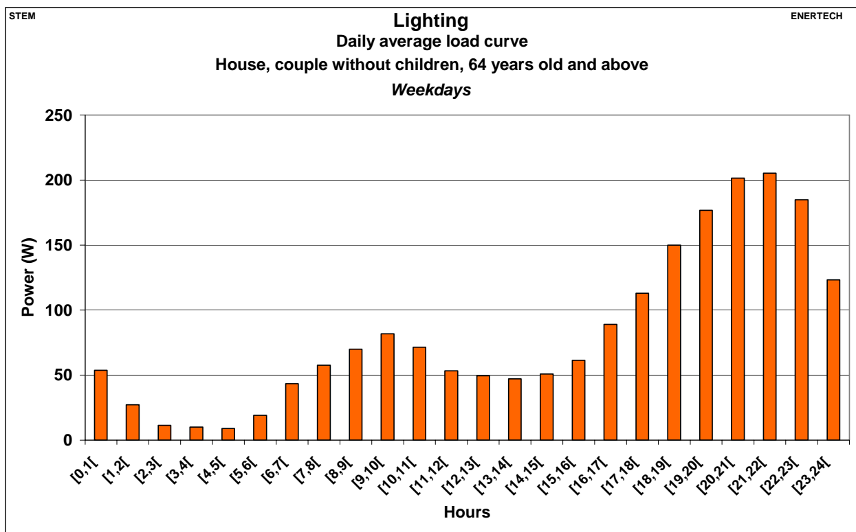
Figure 2.374: Lighting – Daily average load curve – House, couples without children, 64 years old and above – Weekdays
