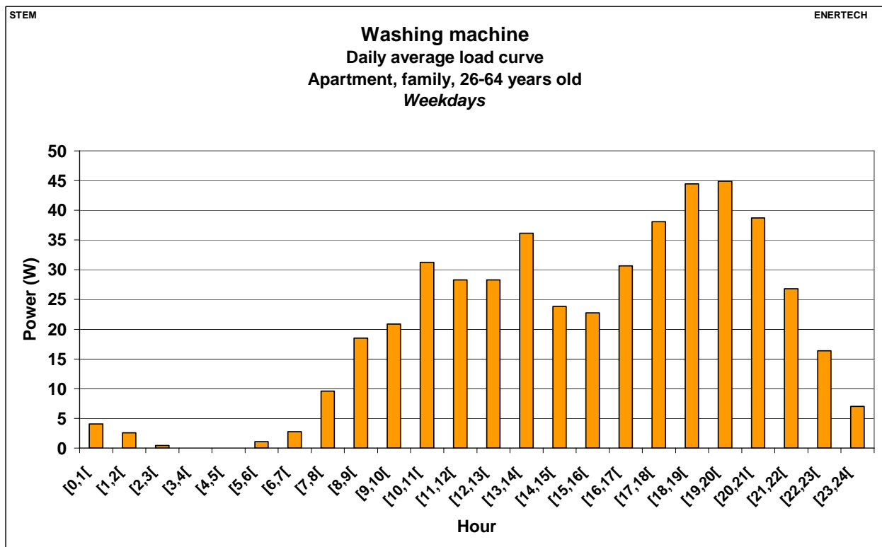
Figure 2.223: Washing machine – Daily average load curve – Apartment, family, 26-64 years old – Weekdays
