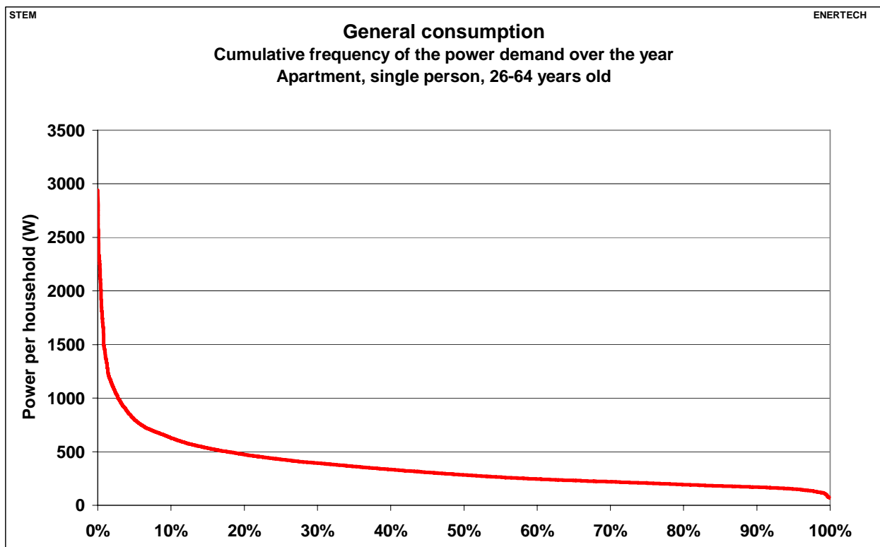
Figure 2.53: General consumption – Cumulative frequency of the power demand over the year, from the grid point of view – Apartment, single person, 26-64 years old
