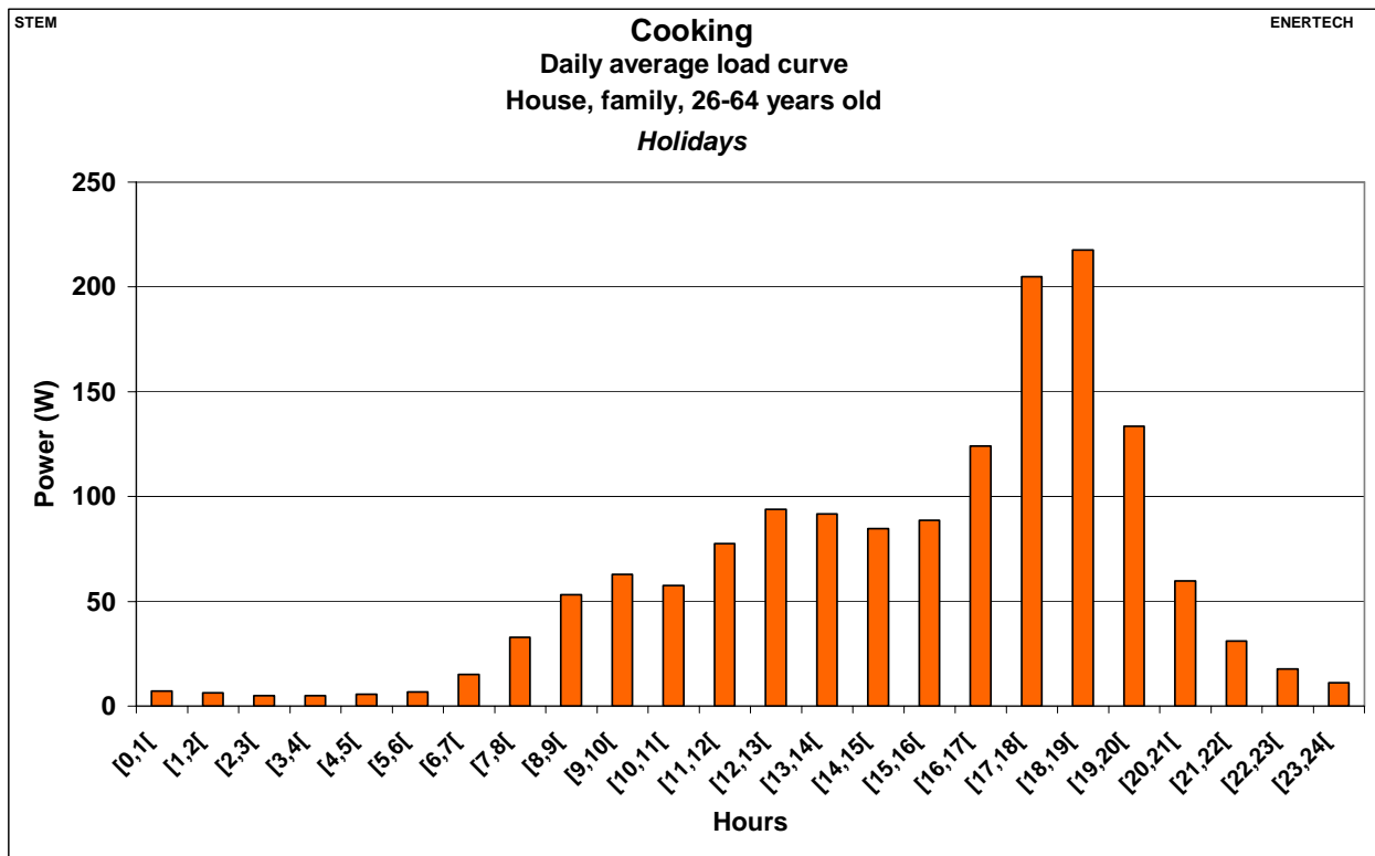
Figure 2.288: Cooking – Daily average load curve – House, family, 26-64 years old – Holidays
