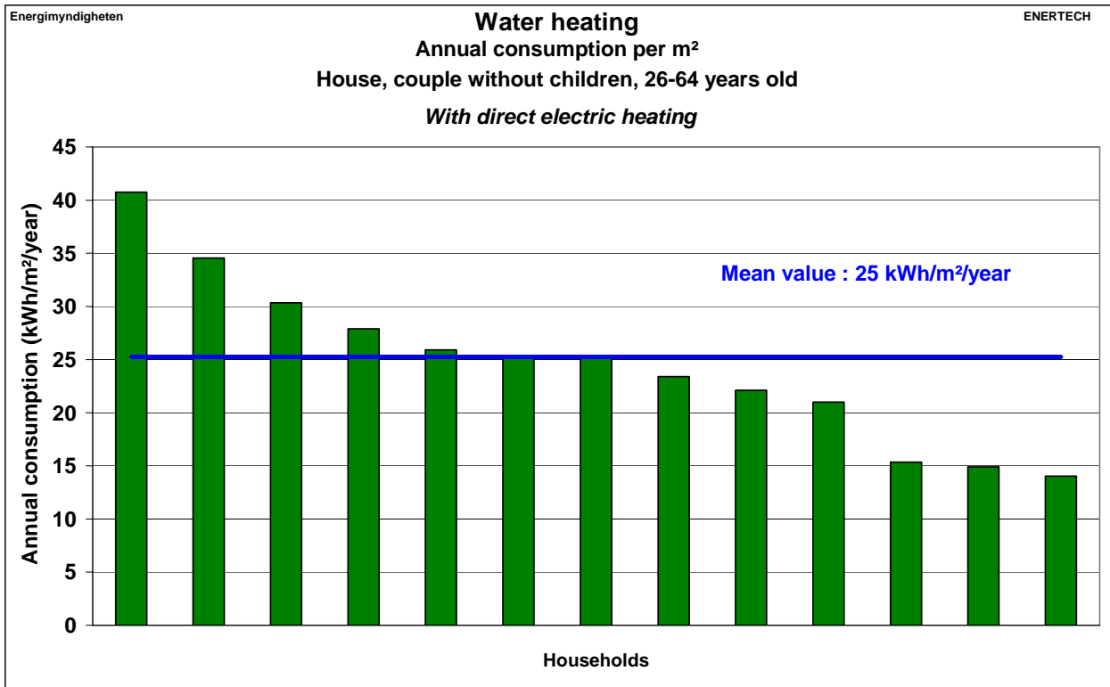
Figure 2.466: Water heating – Annual consumption per m 2 – House, couples without children, 26-64 years old – Direct electric heating
