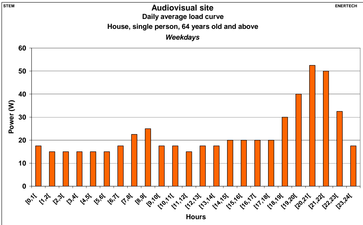
Figure 2.406: Audiovisual site – Daily average load curve – House, single person, 64 years old and above – Weekdays
