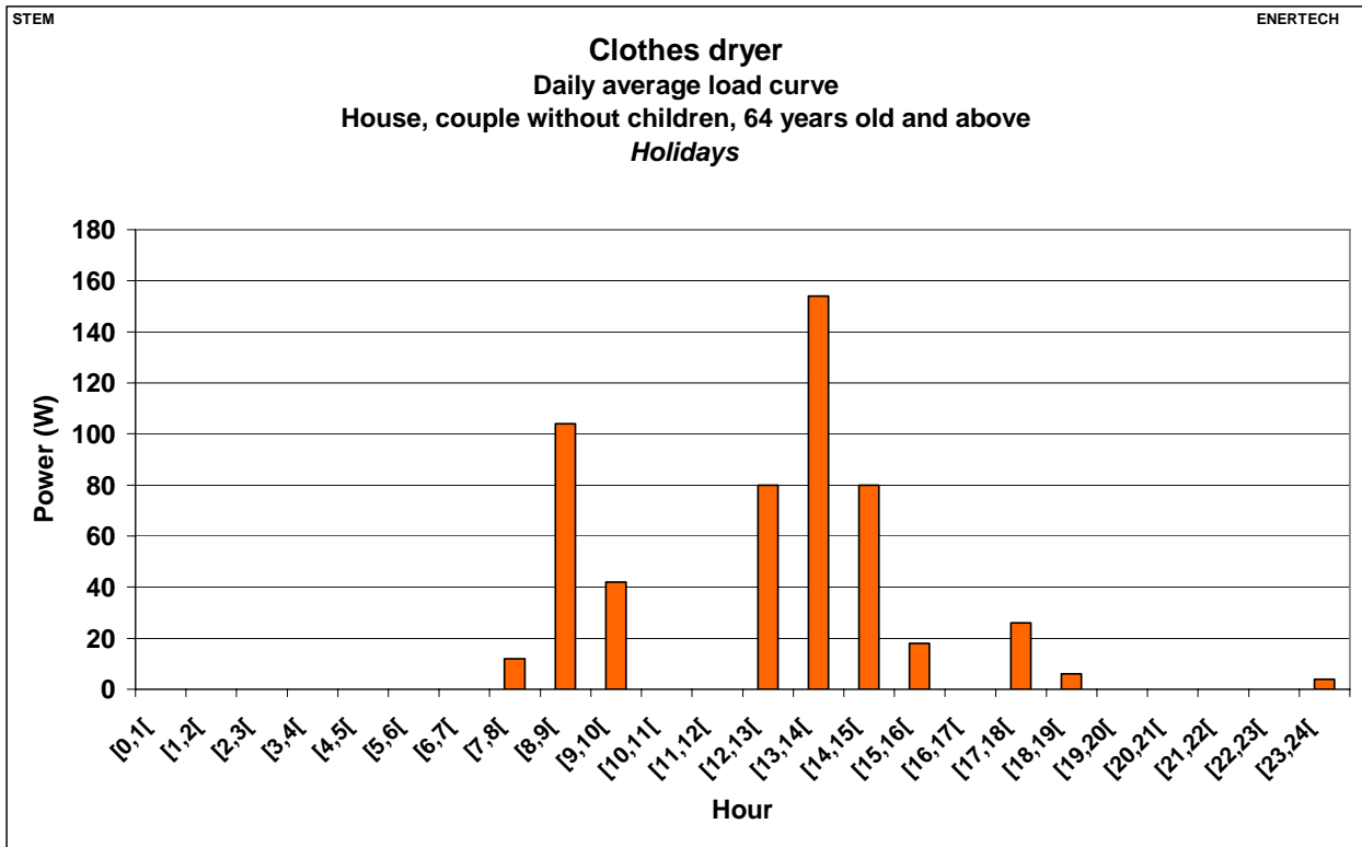
Figure 2.236: Clothes dryer – Daily average load curve – House, couples without children, 64 years old and above – Holidays
