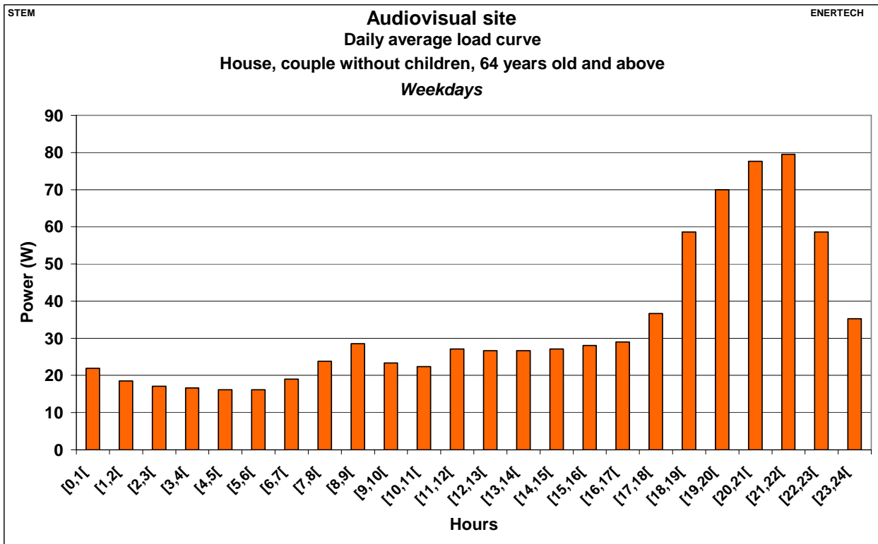
Figure 2.402: Audiovisual site – Daily average load curve – House, couples without children, 64 years old and above – Weekdays
