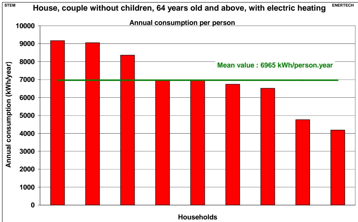
Figures 2.21: Total annualized electricity consumption per person– Houses with electric heating
