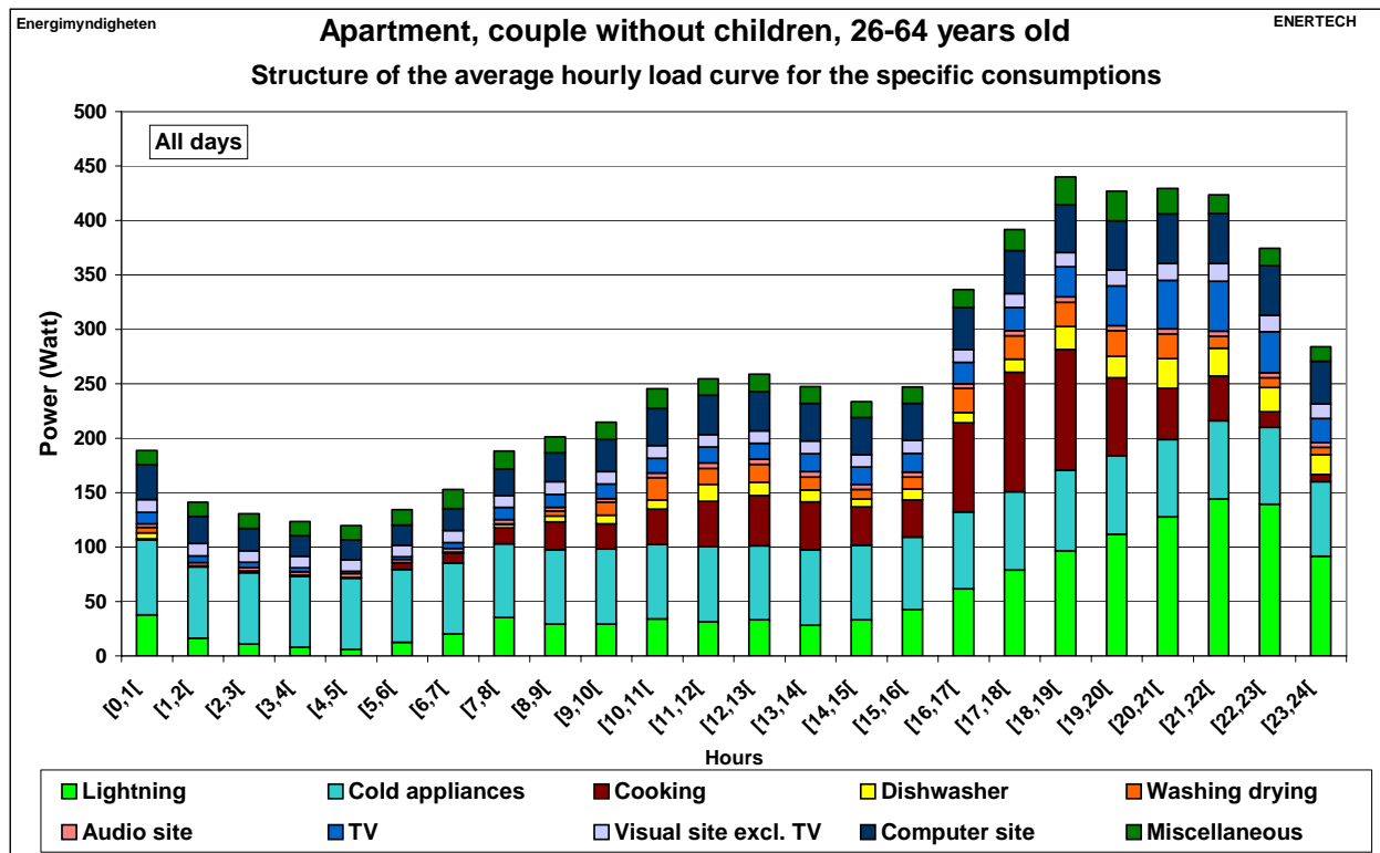
Figure 2.89: Structure of the average hourly load curve for the specific consumption– Apartments – All days
