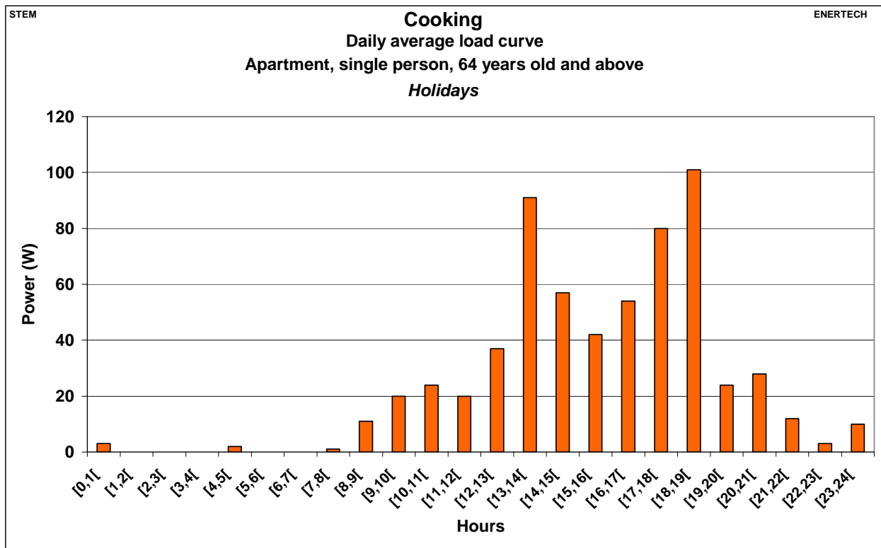
Figure 2.282: Cooking – Daily average load curve – Apartment, single person, 64 years old and above – Holidays
