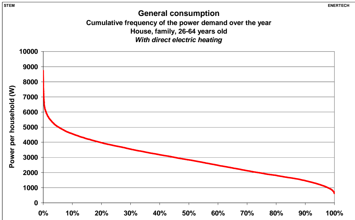
Figure 2.44: General consumption – Cumulative frequency of the power demand over the year, from the grid point of view – House, family, 26-64 years old - With direct electric heating
