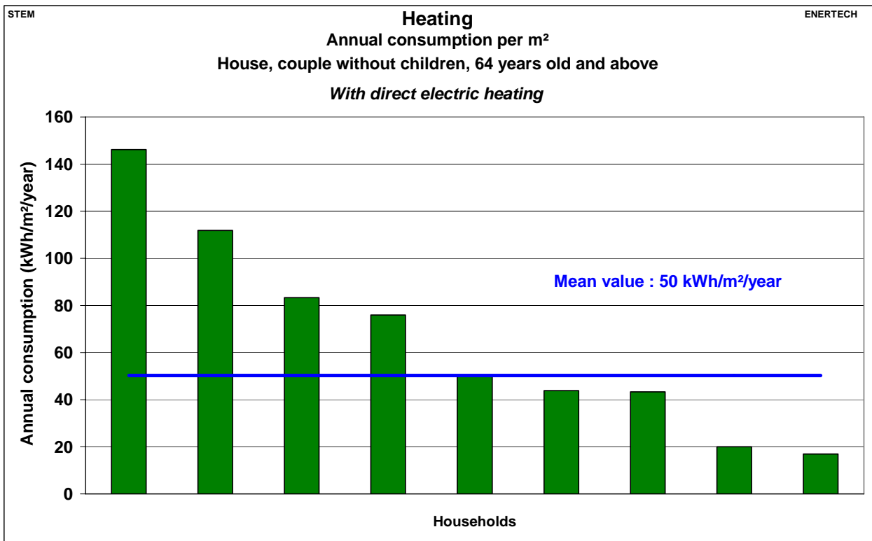
Figure 2.461: Heating – Annual consumption per m 2 – House, couples without children, 64 years old and above –Direct electric heating
