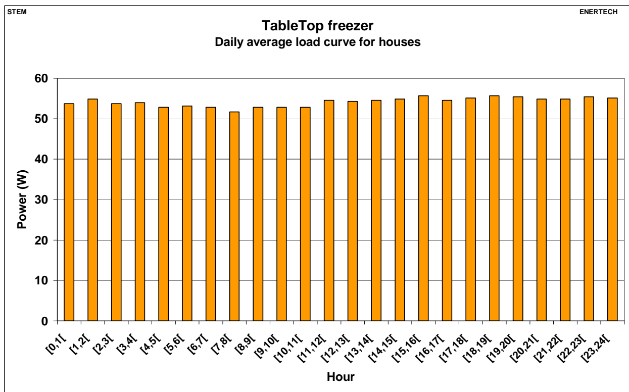
Figure 2.202: TableTop freezer: daily average load curves – all households
