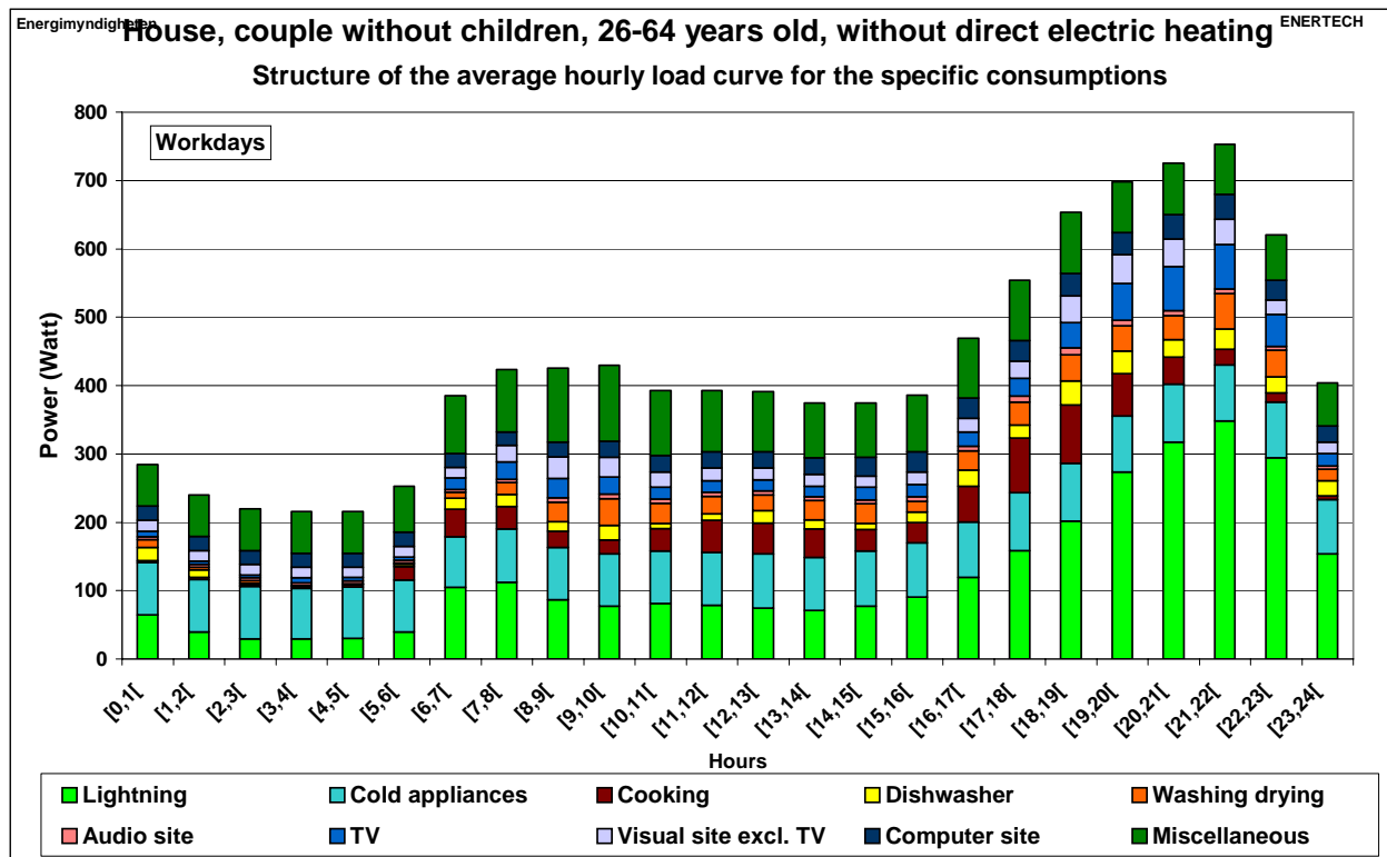
Figure 2.85: Structure of the average hourly load curve for the specific consumption– Houses without direct electric heating – Workdays
