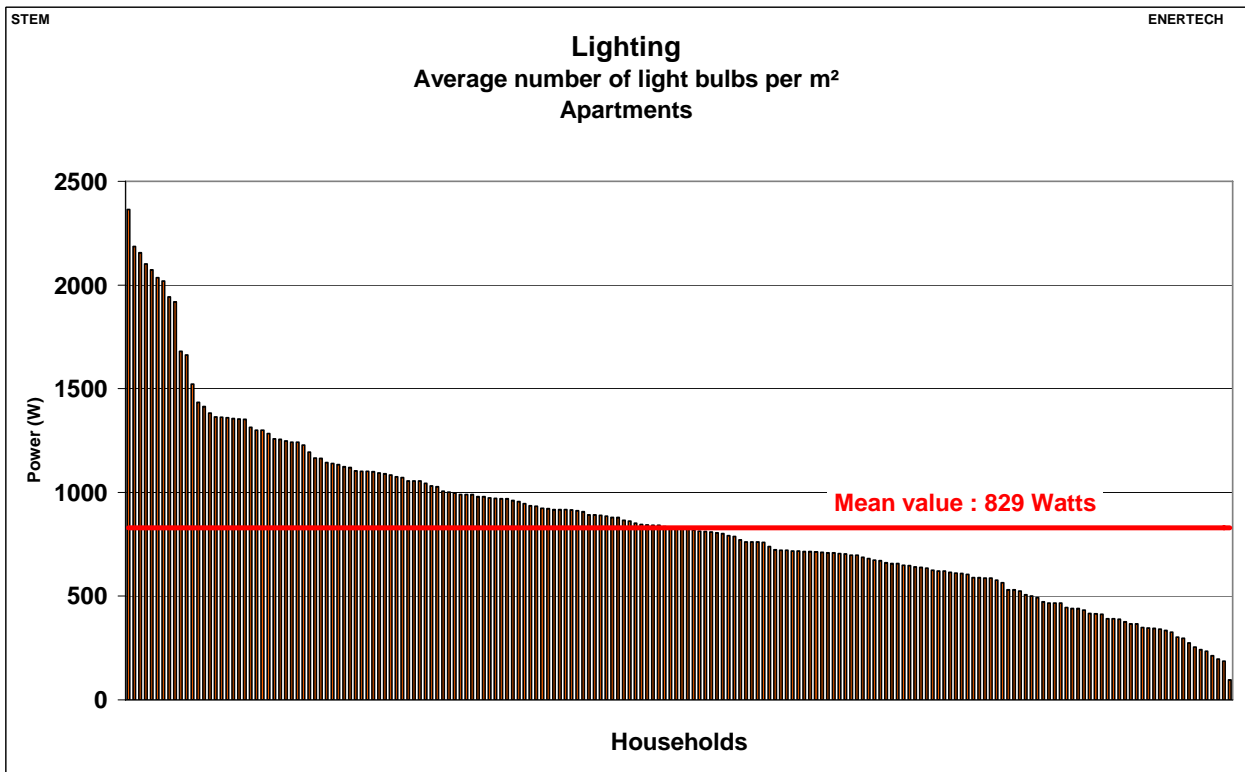
Figure 2.323: Lighting – Average value for the installed lighting wattage – Apartments
