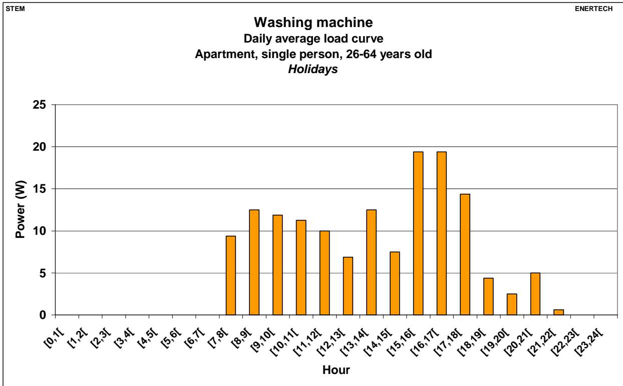
Figure 2.224: Washing machine – Daily average load curve – Apartment, single person, 26-64 years old – Holidays
