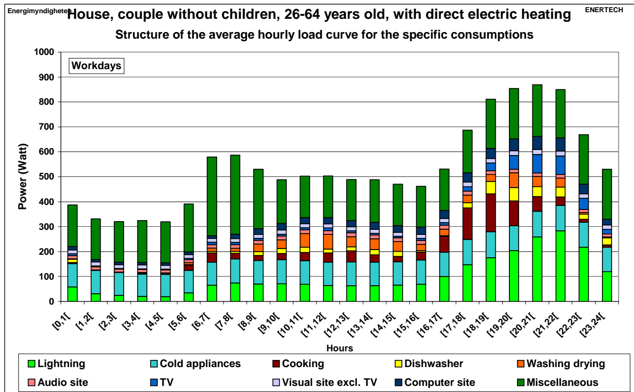
Figure 2.79: Structure of the average hourly load curve for the specific consumption– Houses with direct electric heating – Workdays
