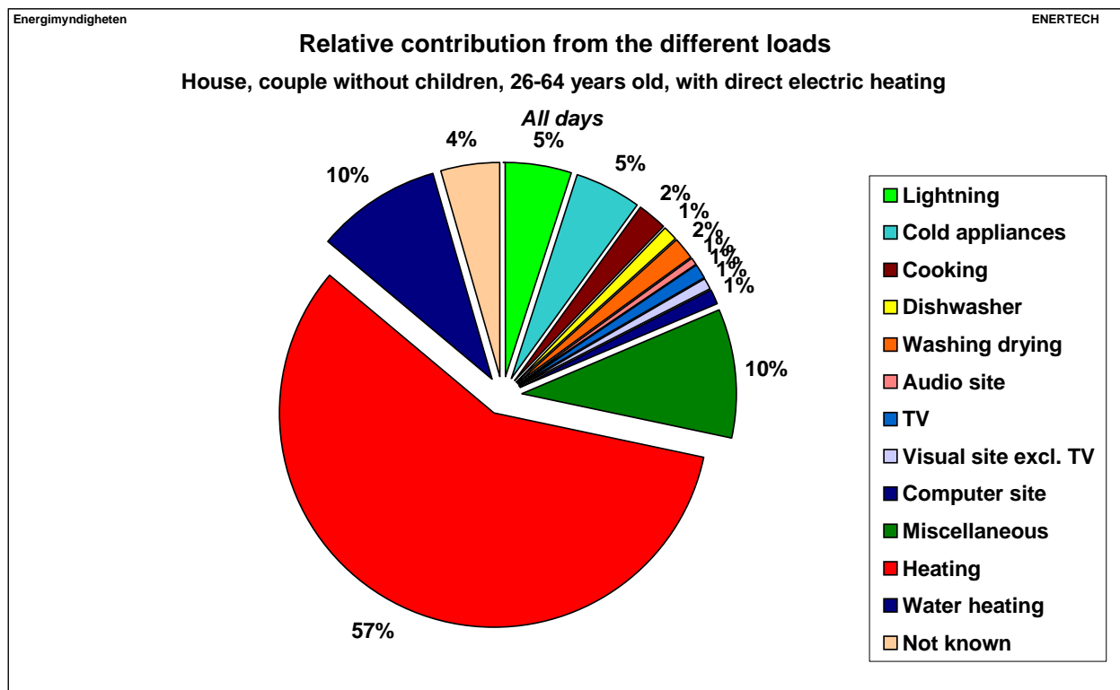
Figure 2.140: Relative contribution from the different loads – Houses with direct electric heating – All days
