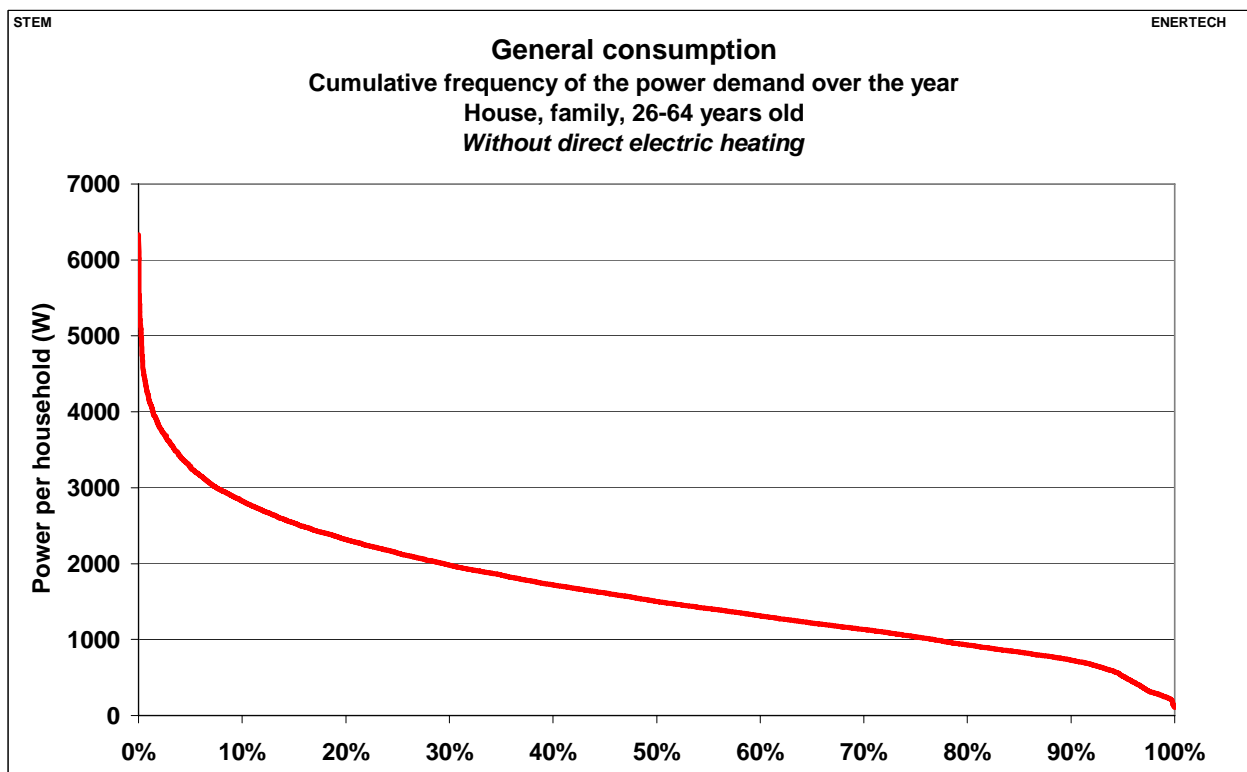
Figure 2.45: General consumption – Cumulative frequency of the power demand over the year, from the grid point of view – House, family, 26-64 years old - Without direct electric heating
