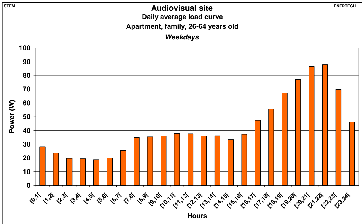
Figure 2.394: Audiovisual site – Daily average load curve – Apartment, family, 26-64 years old – Weekdays
