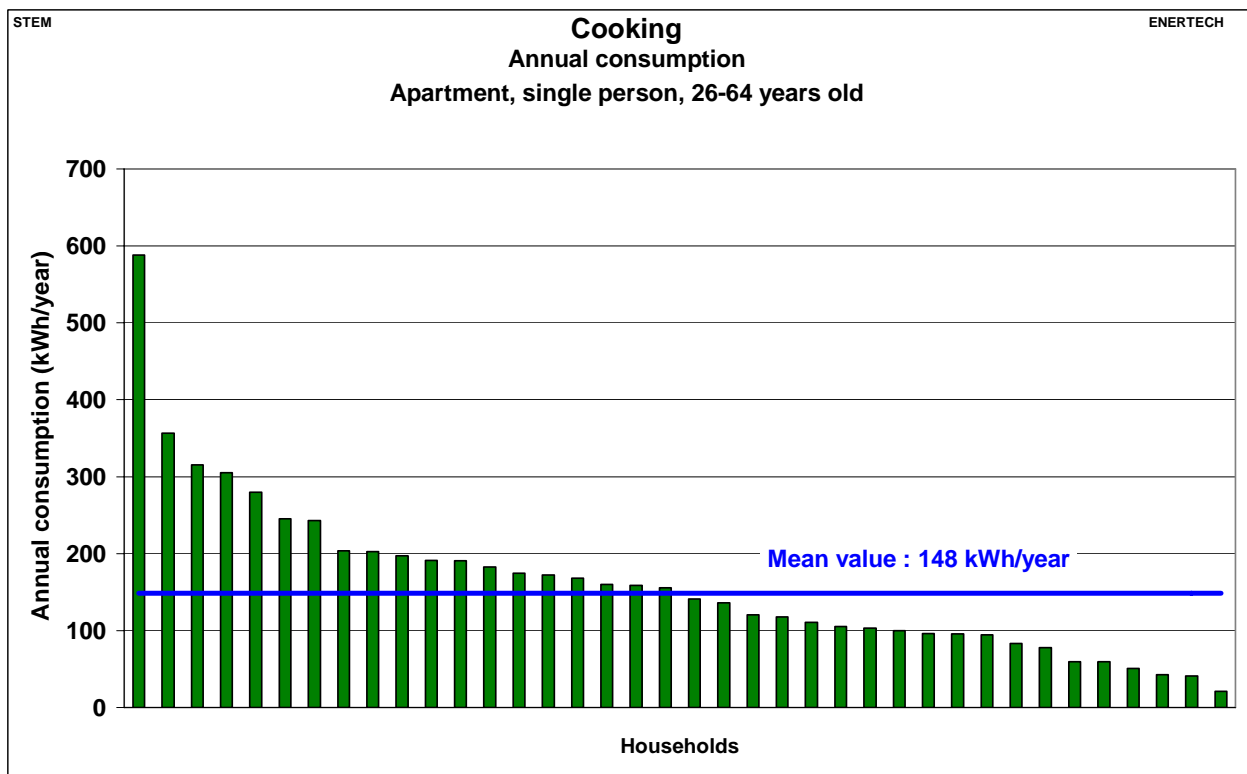
Figure 2.271: Cooking – Annual consumption – Apartment, single person, 26-64 years old
