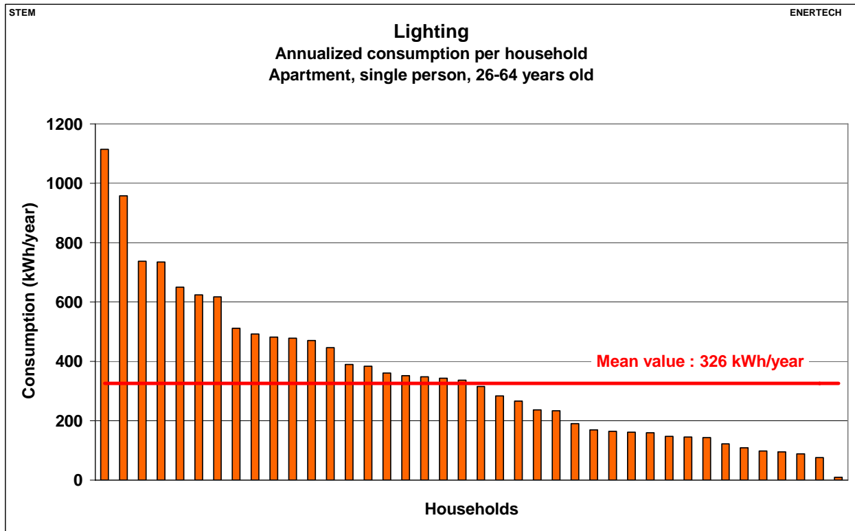
Figure 2.352: Lighting – Annualized consumption – Apartment, single person, 26-64 years old
